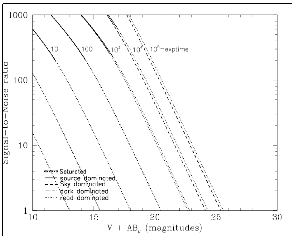
Figure 10.63: Extended source S/N vs. V+AB for the HRC/F502N filter. Top curves are for low sky and bottom curves are for average sky for a 1 arcsec 2 area.
