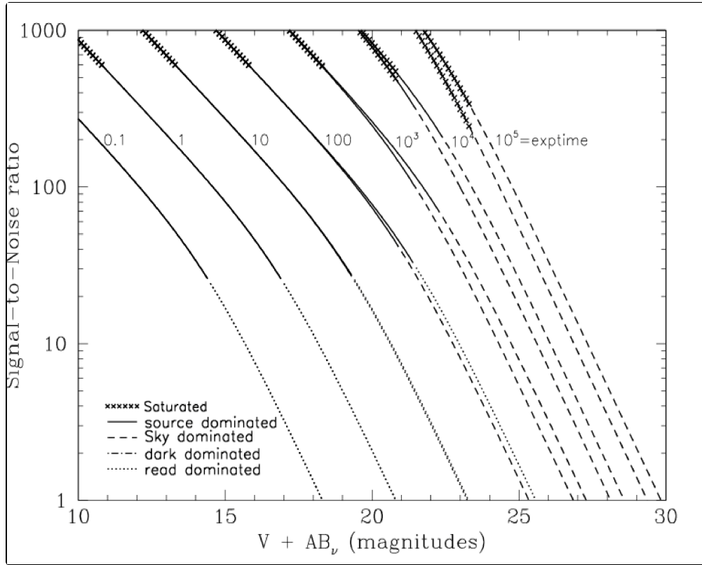
Figure 10.11: Point source S/N vs. V+AB for the WFC/F550M filter. Top curves are for low sky; bottom curves are for average sky.
