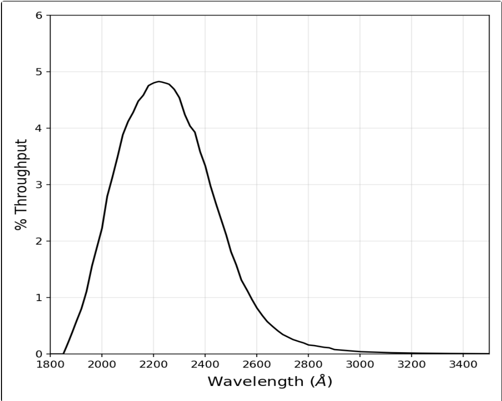
Figure 10.43: Integrated system throughput for HRC/F220W.
