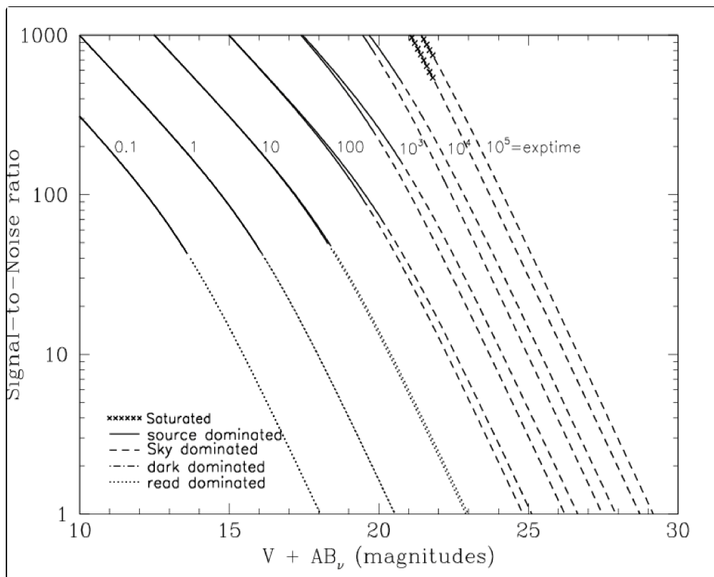
Figure 10.86: Point source S/N vs. V+AB for the HRC/F814W filter. Top curves are for low sky; bottom curves are for average sky.
