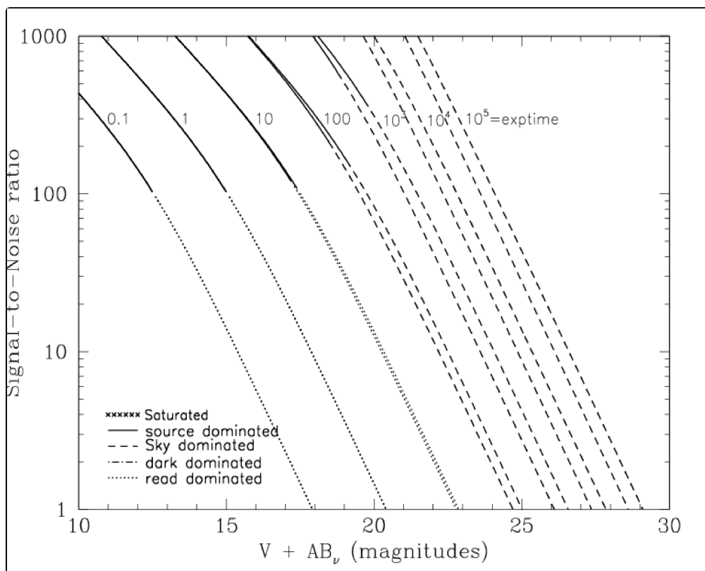
Figure 10.6: Extended source S/N vs. V+AB for the WFC/F475W filter. Top curves are for low sky and bottom curves are for average sky for a 1 arcsec 2 area.
