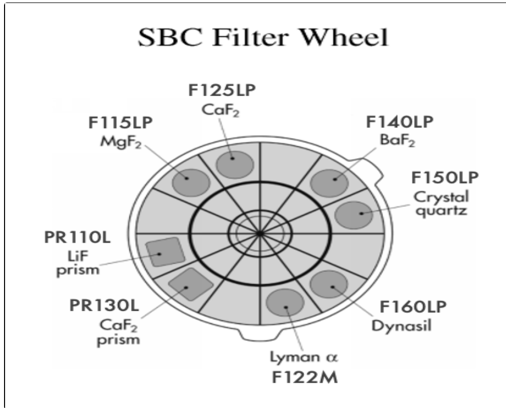
Figure 5.12: SBC Filter wheel layout
