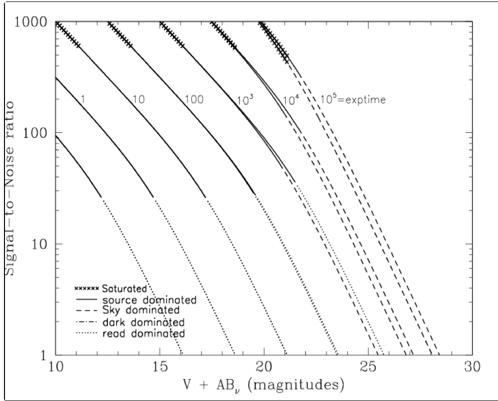
Figure 10.23: Point source S/N vs. V+AB for the WFC/F658N filter. Top curves are for low sky; bottom curves are for average sky.
