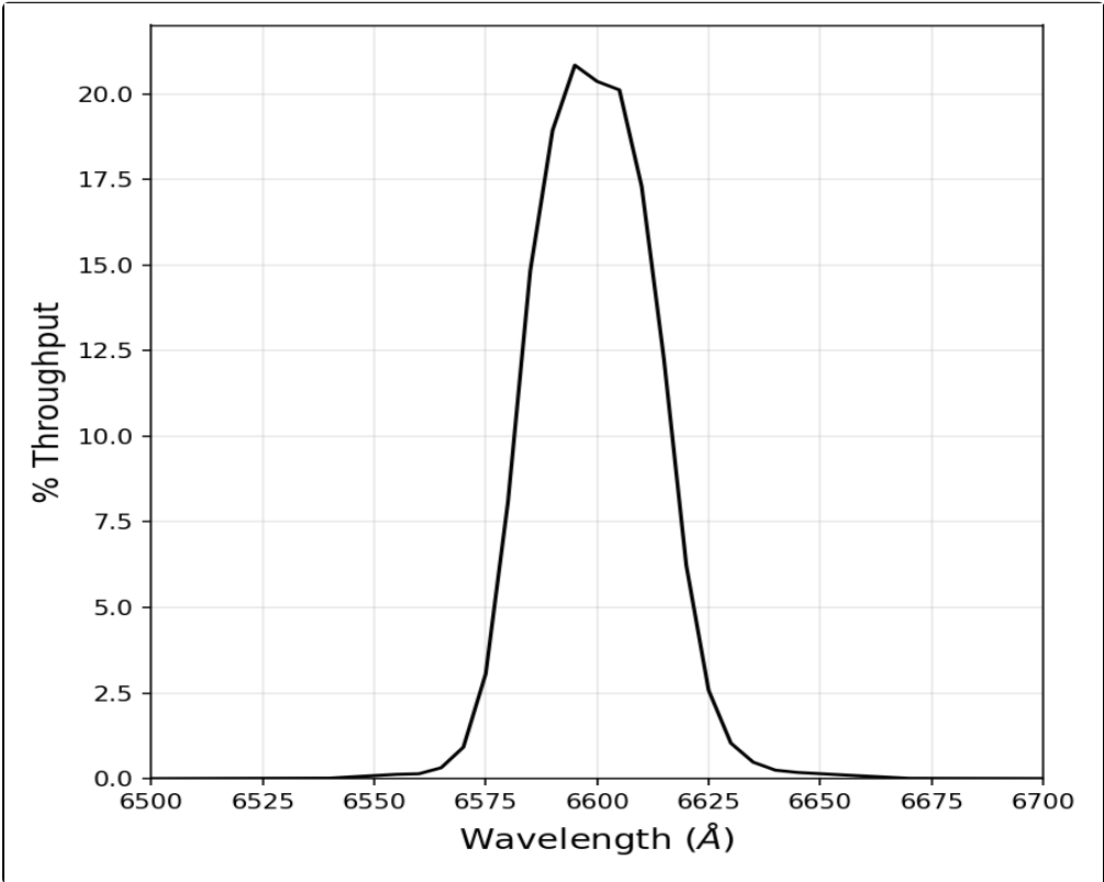
Figure 10.79: Integrated system throughput for HRC/F660N.
