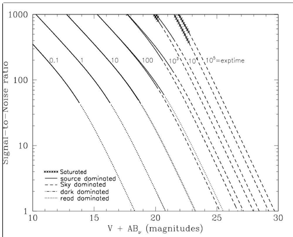
Figure 10.59: Point source S/N vs. V+AB for the HRC/F475W filter. Top curves are for low sky; bottom curves are for average sky.
