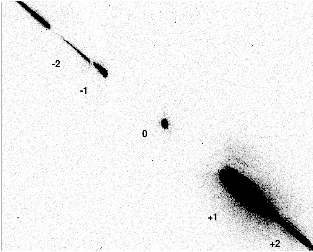
The numbers indicate the different grism orders.
