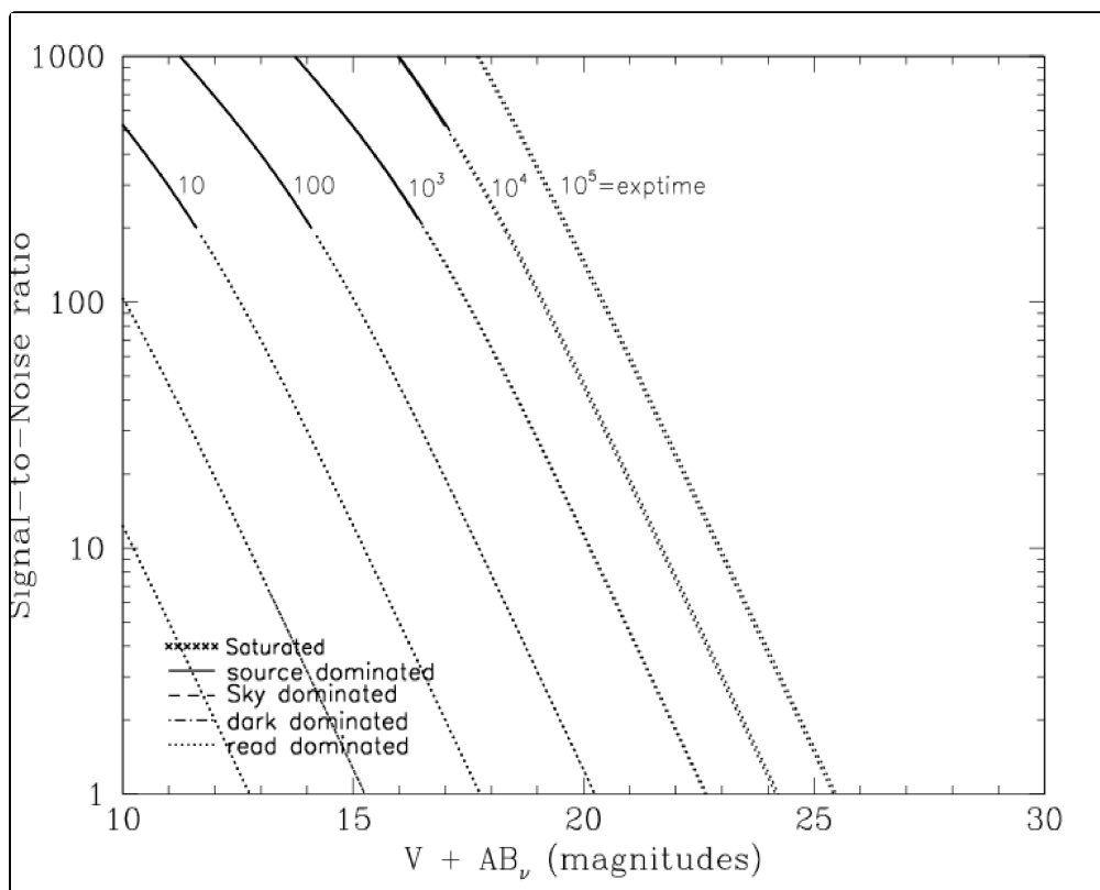
Figure 10.54: Extended source S/N vs. V+AB for the HRC/F344N filter. Top curves are for low sky and bottom curves are for average sky for a 1 arcsec 2 area.
