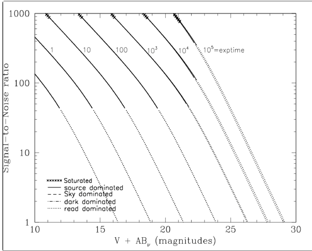
Figure 10.44: Point source S/N vs. V+AB for the HRC/F220W filter. Top curves are for low sky; bottom curves are for average sky.
