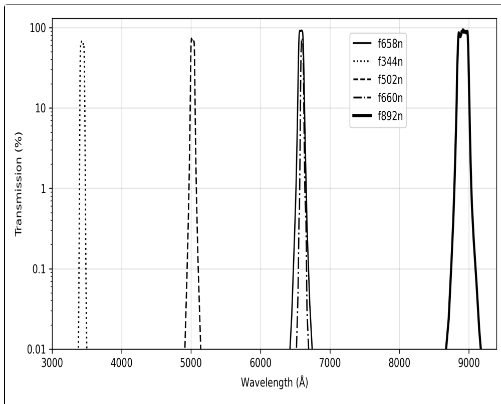
Figure 5.4: ACS narrow band filters.
