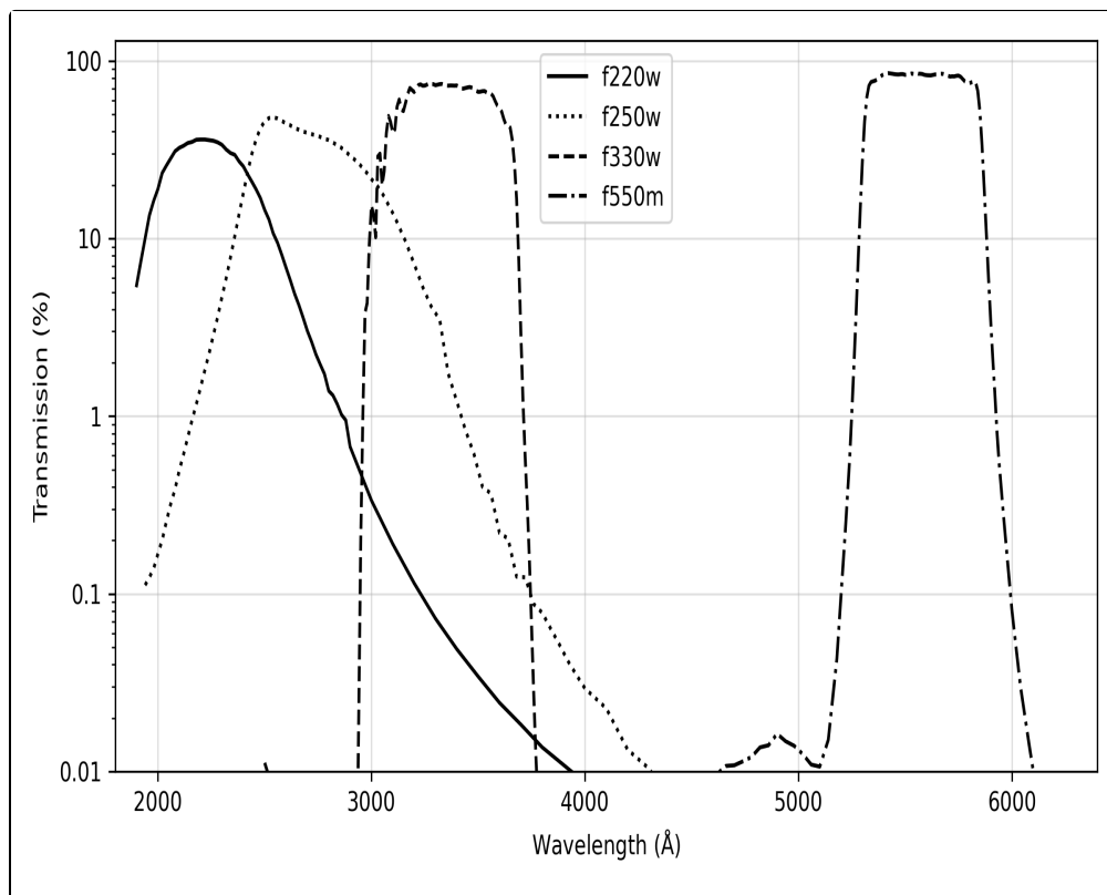
Figure 5.3: ACS UV and medium-band filters.
