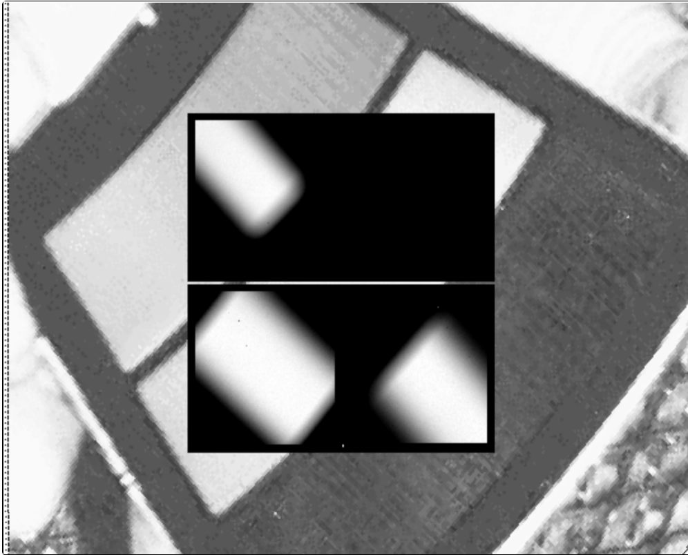
Figure 7.5: Monochromatic patches in ground calibration data showing actual aperture sizes through ramp filters (superimposed on photo of ramp filters).
