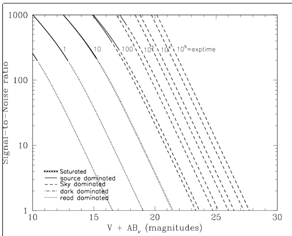
Figure 10.75: Extended source S/N vs. V+AB for the HRC/F625W filter. Top curves are for low sky and bottom curves are for average sky for a 1 arcsec 2 area.
