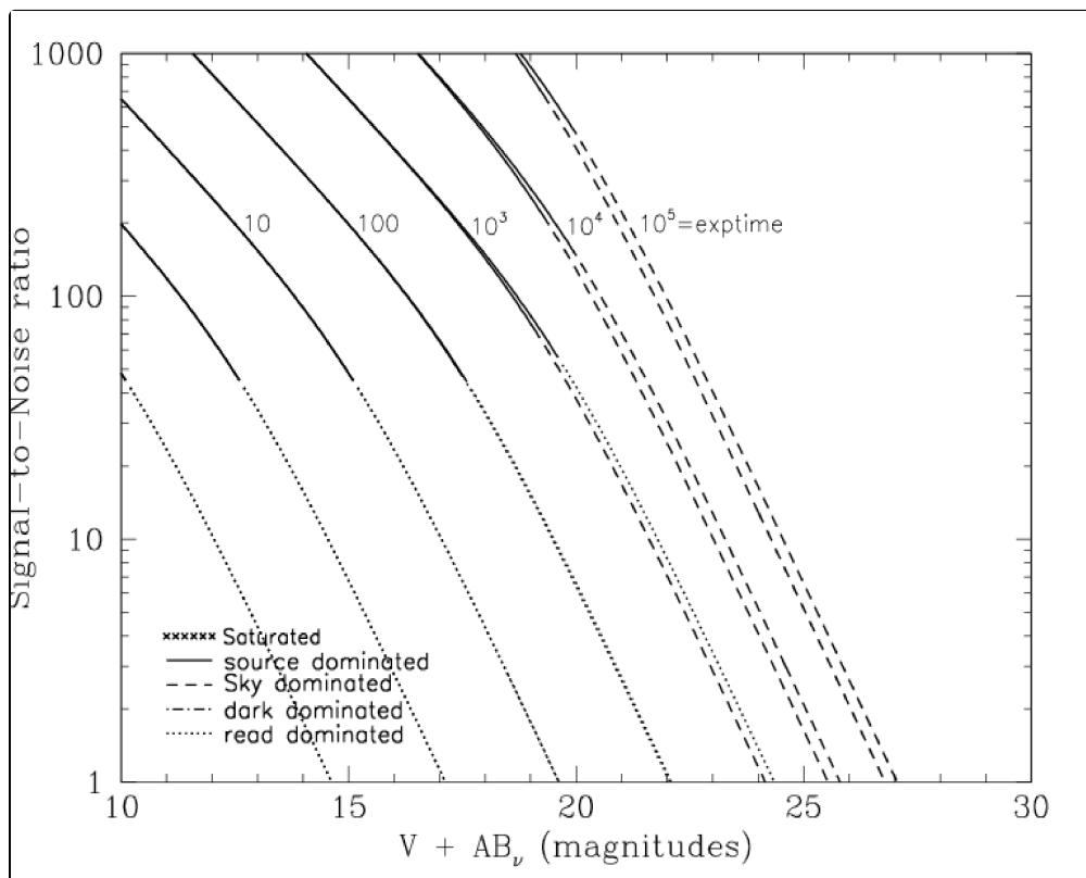
Figure 10.92: Point source S/N vs. V+AB for the HRC/F892N filter. Top curves are for low sky; bottom curves are for average sky.
