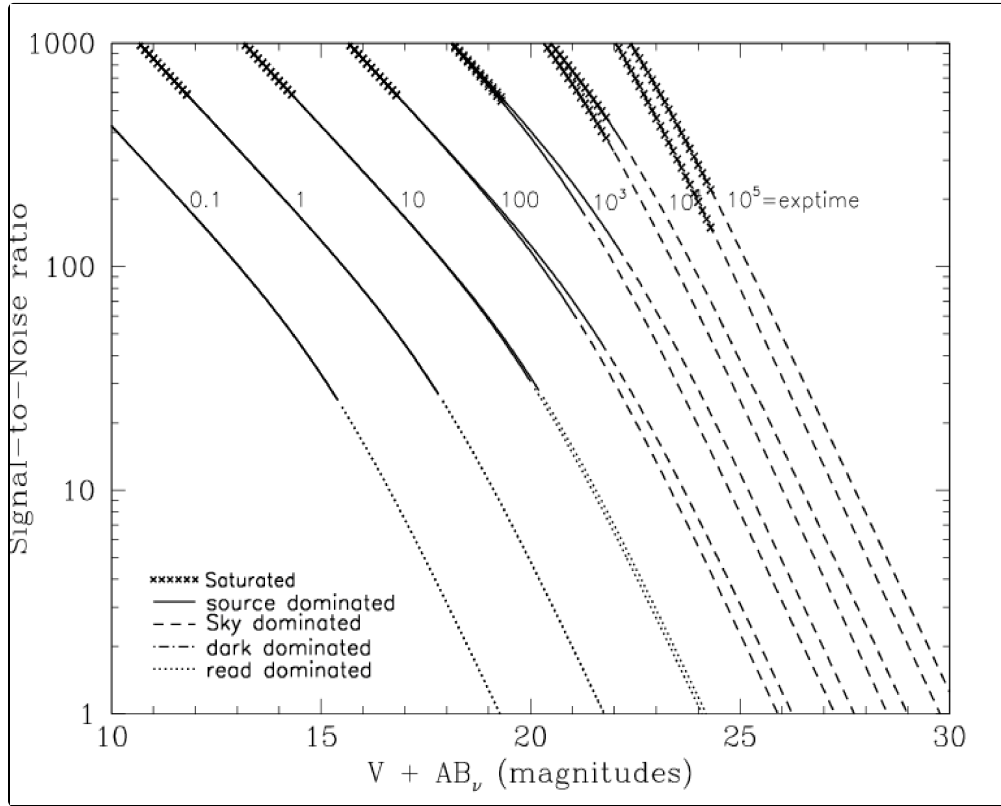
Figure 10.20: Point source S/N vs. V+AB for the WFC/F625W filter. Top curves are for low sky; bottom curves are for average sky.
