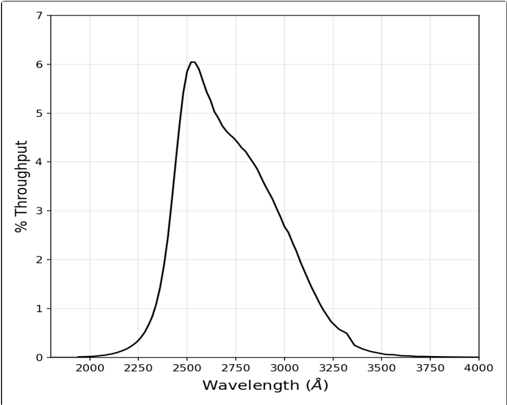
Figure 10.46: Integrated system throughput for HRC/F250W.
