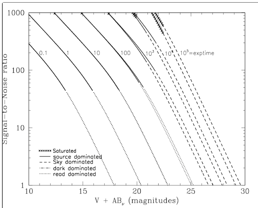
Figure 10.56: Point source S/N vs. V+AB for the HRC/F435W filter. Top curves are for low sky; bottom curves are for average sky.
