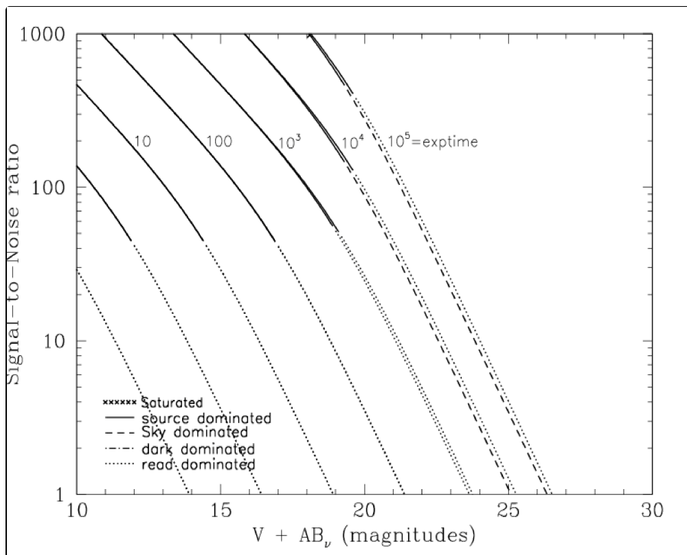
Figure 10.80: Point source S/N vs. V+AB for the HRC/F660N filter. Top curves are for low sky; bottom curves are for average sky.
