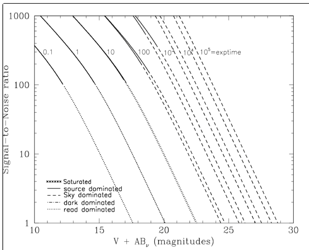
Figure 10.15: Extended source S/N vs. V+AB for the WFC/F555W filter. Top curves are for low sky and bottom curves are for average sky for a 1 arcsec 2 area.
