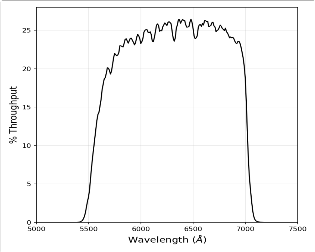
Figure 10.73: Integrated system throughput for HRC/F625W.
