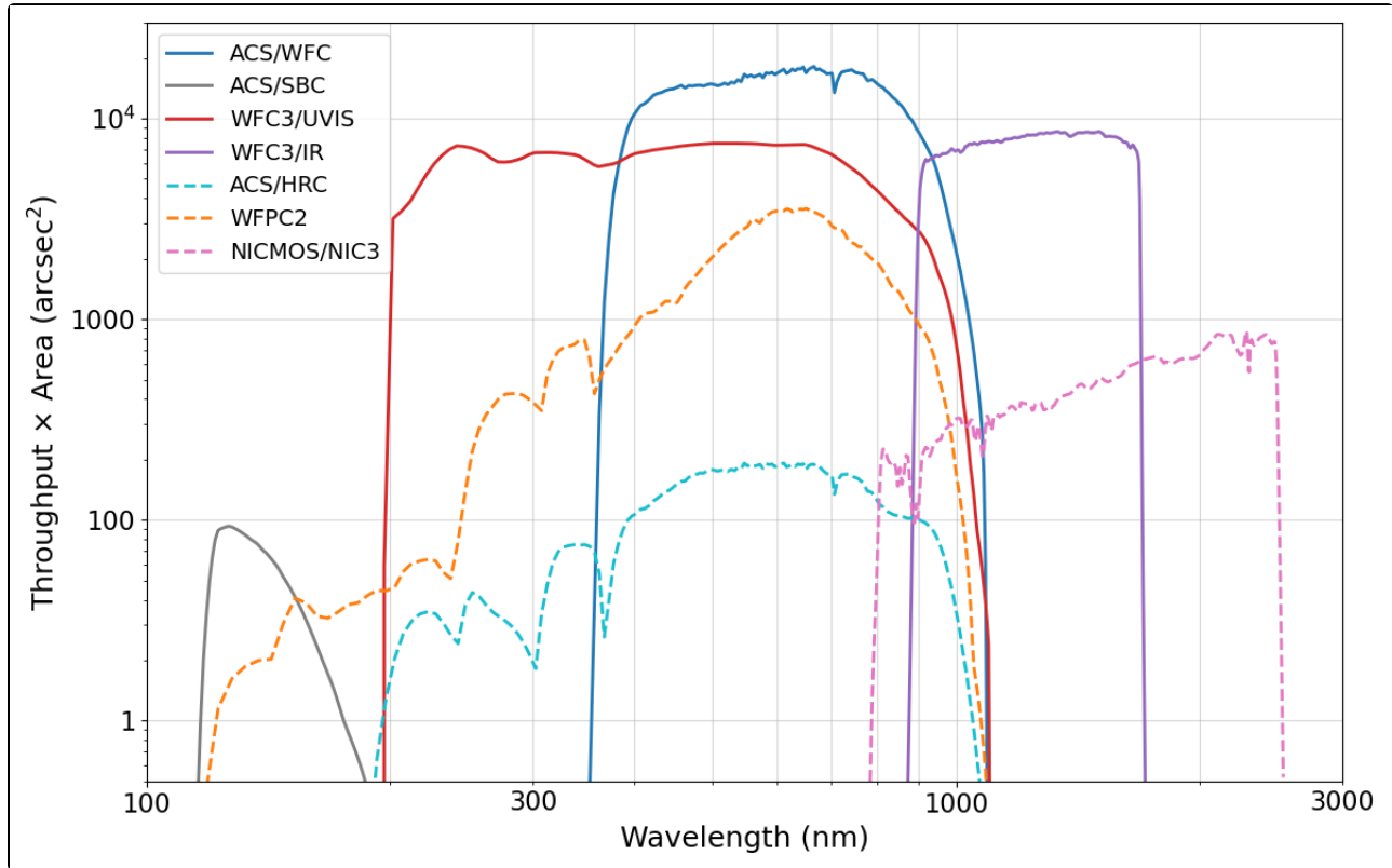
HST survey discovery efficiencies of the cameras, defined as the system throughput multiplied by the area of the field-of-view. Solid lines represent instruments currently active on board HST . Dashed lines represent instruments that are no longer offered ( HRC , NICMOS ) and a previously flown instrument ( WFPC2 ).
