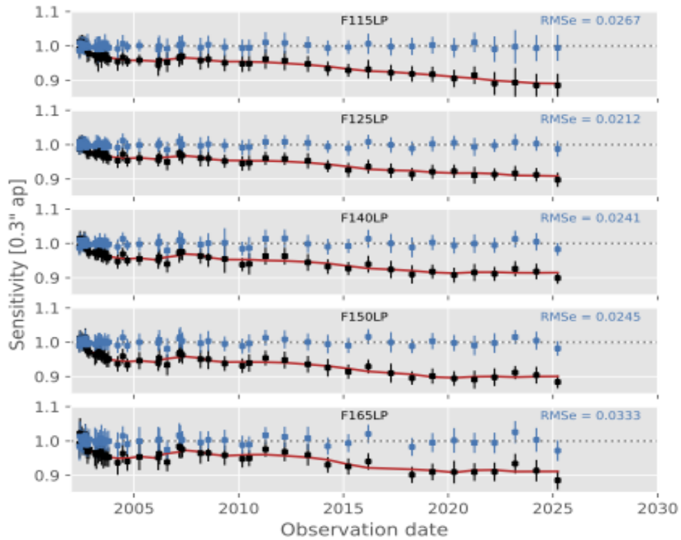
Figure 4.20: Sensitivity of five of the SBC imaging modes as a function of time
