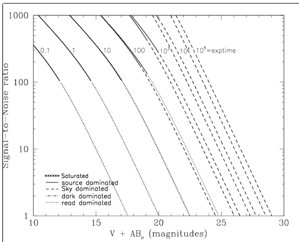
Figure 10.3: Extended source S/N vs. V+AB for the WFC/F435W filter. Top curves are for low sky and bottom curves are for average sky for a 1 arcsec 2 area.
