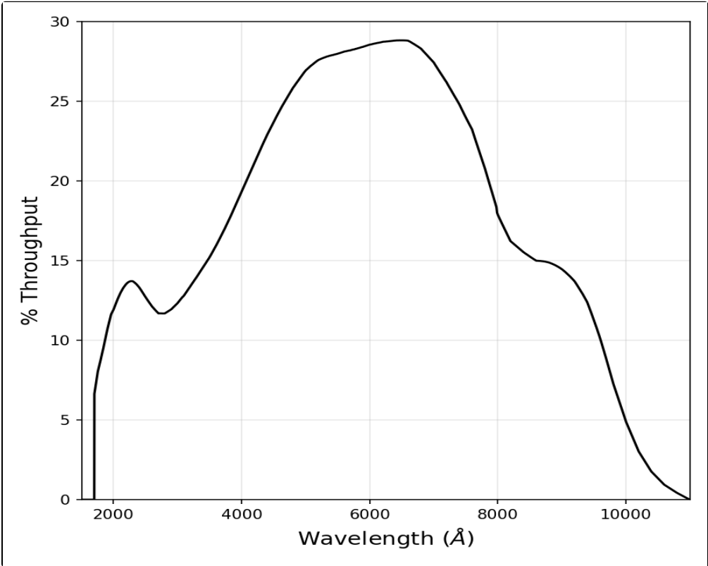
Figure 10.100: Integrated system throughput for HRC/Clear.
