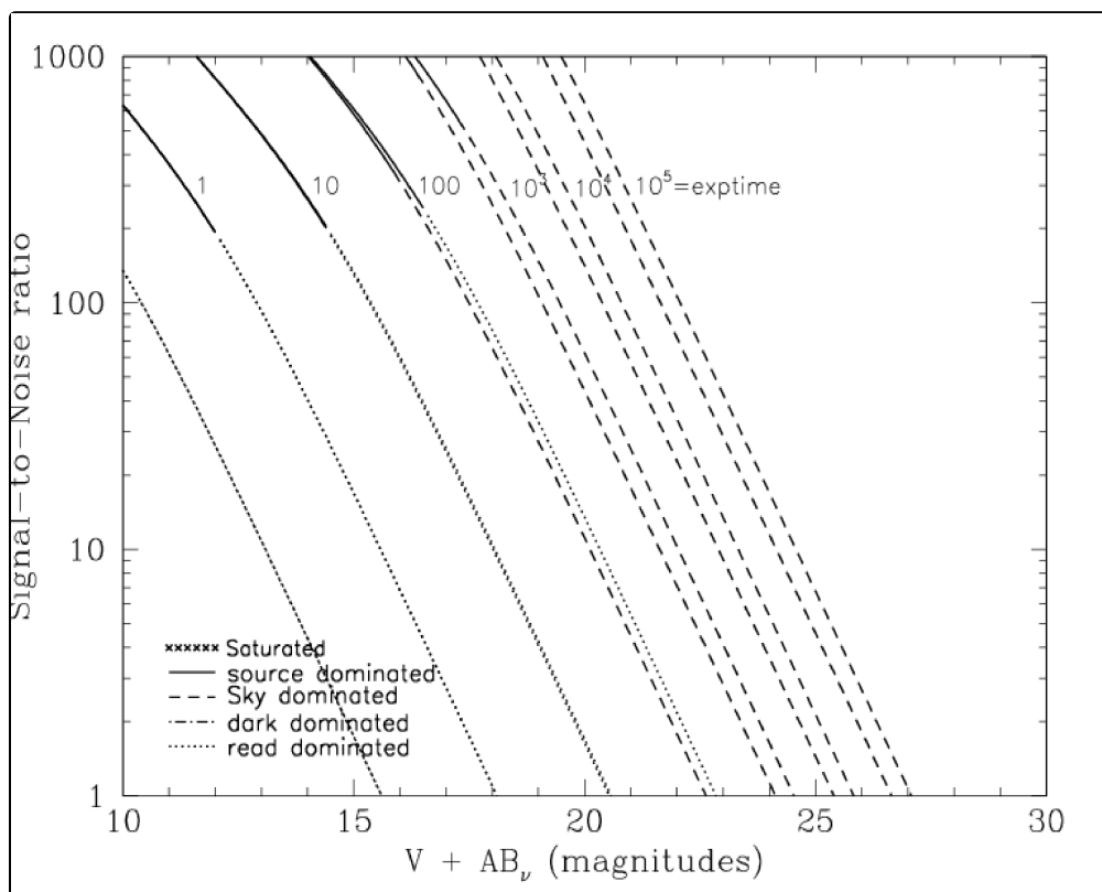
Figure 10.90: Extended source S/N vs. V+AB for the HRC/F850LP filter. Top curves are for low sky and bottom curves are for average sky for a 1 arcsec 2 area.
