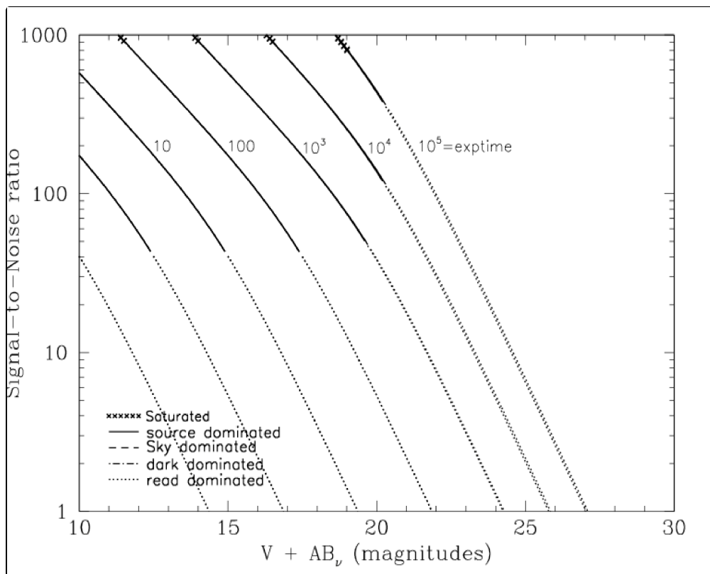
Figure 10.53: Point source S/N vs. V+AB for the HRC/F344N filter. Top curves are for low sky; bottom curves are for average sky.
