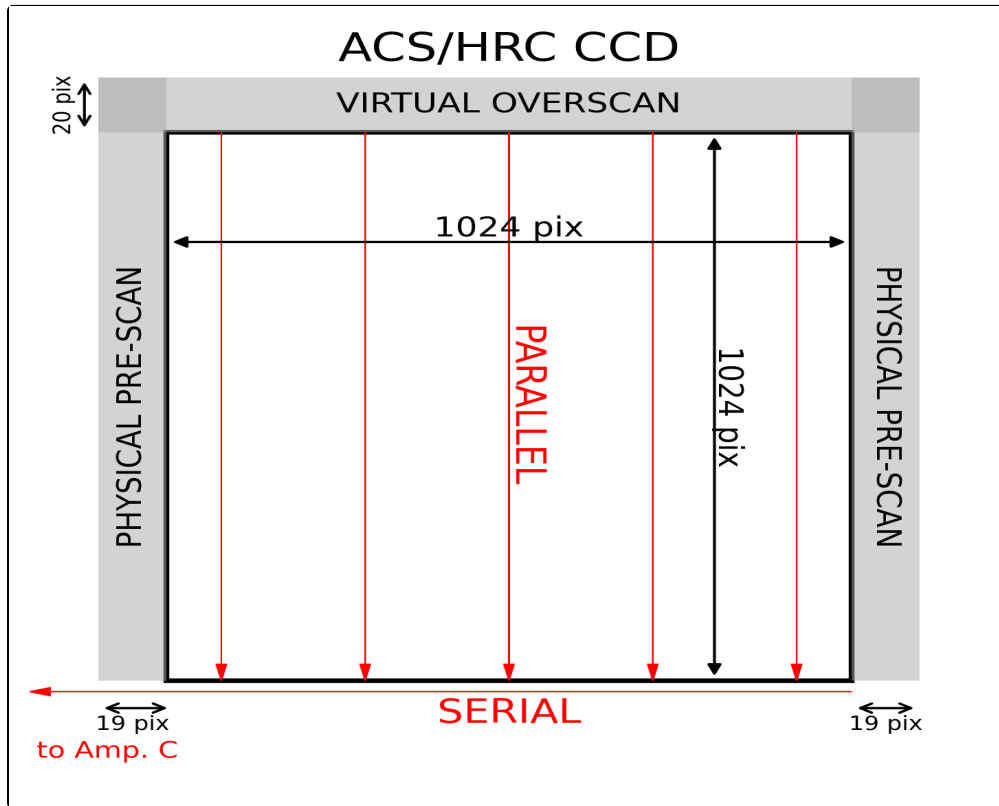
Figure 4.3: The layout of HRC images, including the prescans and overscans.
