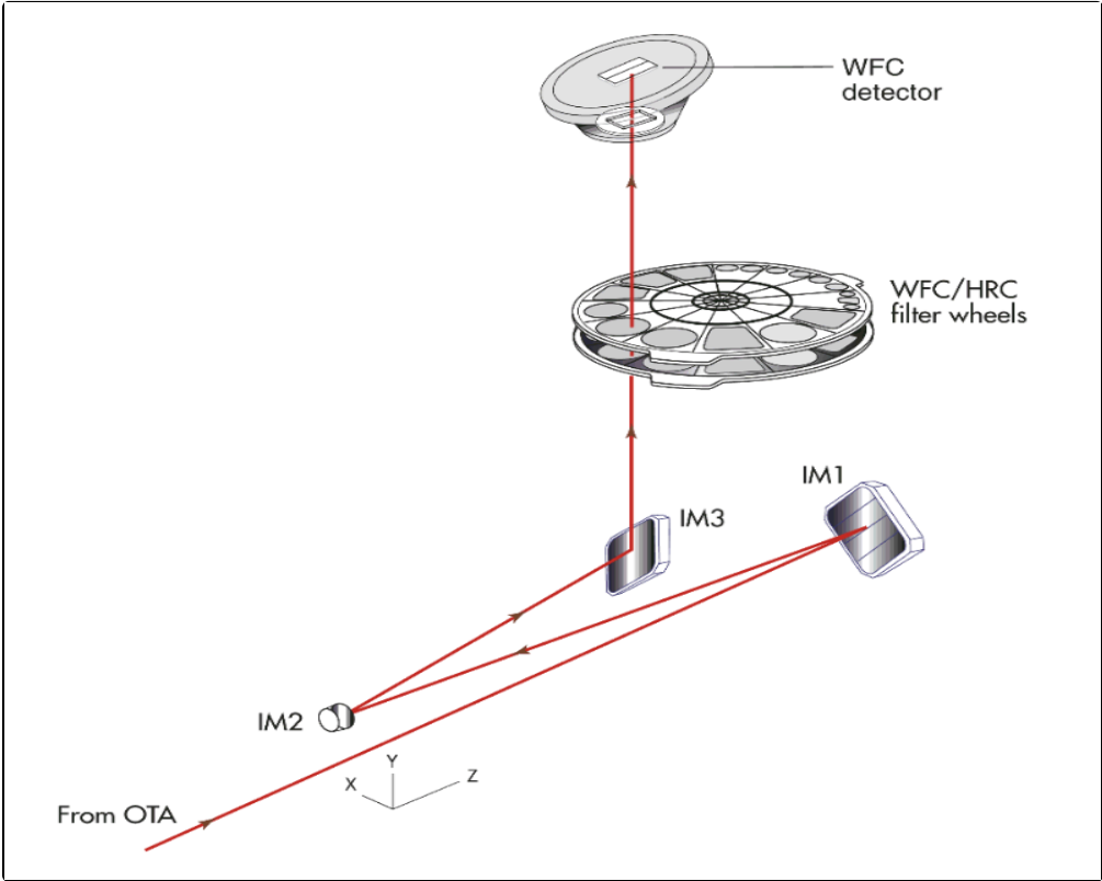
Figure 3.2: ACS optical design: Wide Field Channel (ACS/WFC).
