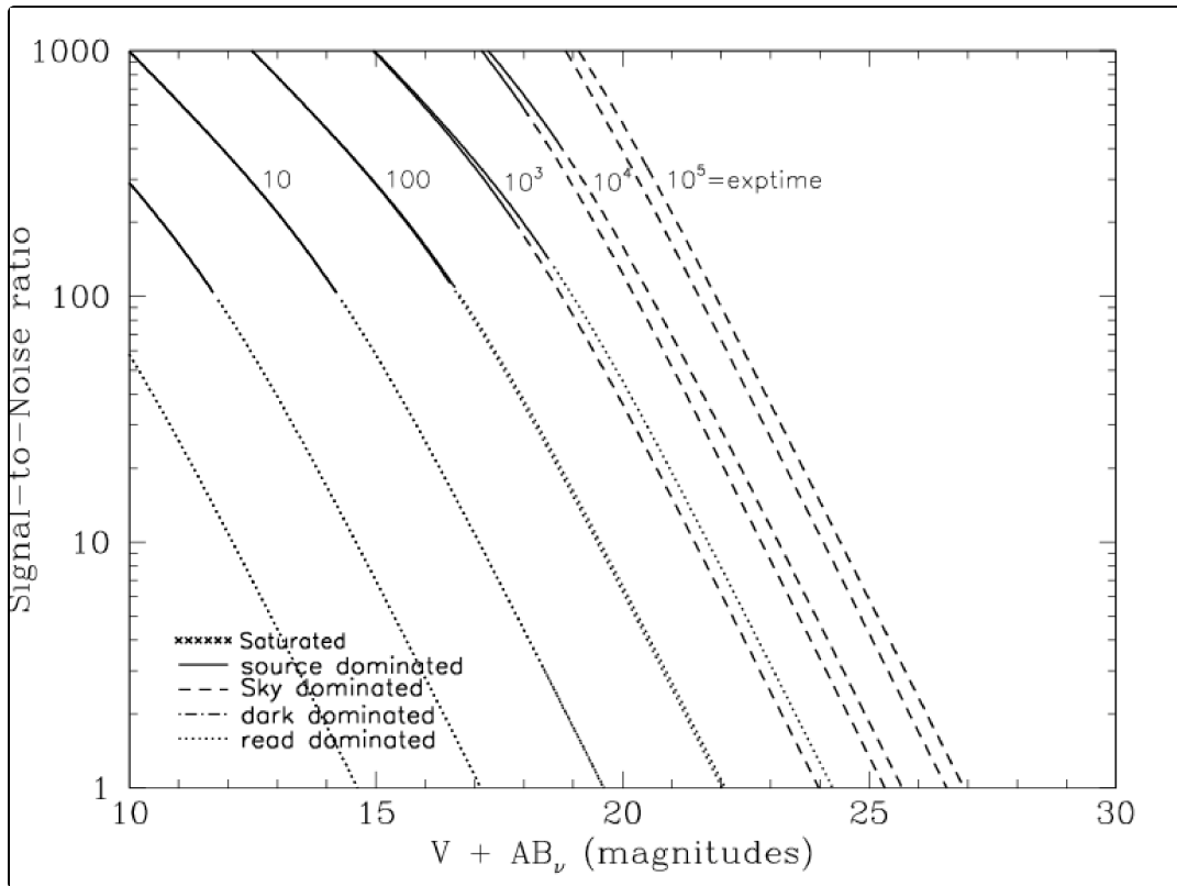
Figure 10.24: Extended source S/N vs. V+AB for the WFC/F658N filter. Top curves are for low sky and bottom curves are for average sky for 1 \text{ arcsec}^2 area.
