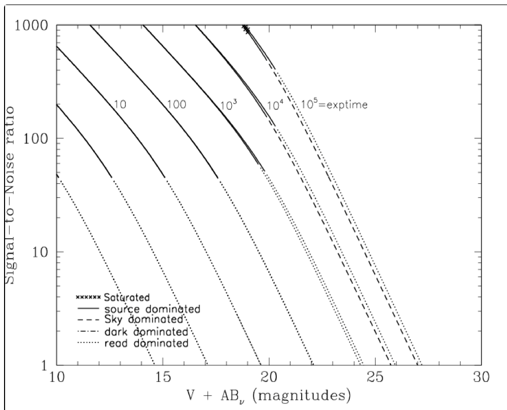
Figure 10.62: Point source S/N vs. V+AB for the HRC/F502N filter. Top curves are for low sky; bottom curves are for average sky.
