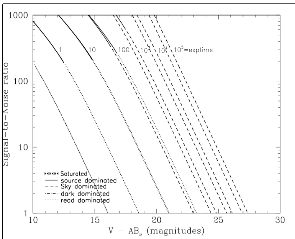
Figure 10.84: Extended source S/N vs. V+AB for the HRC/F775W filter. Top curves are for low sky and bottom curves are for average sky for a 1 arcsec 2 area.
