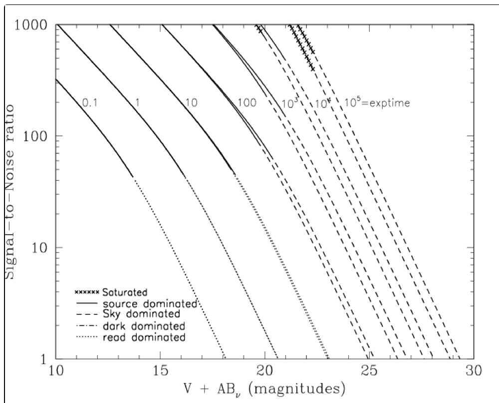
Figure 10.74: Point source S/N vs. V+AB for the HRC/F625W filter. Top curves are for low sky; bottom curves are for average sky.
