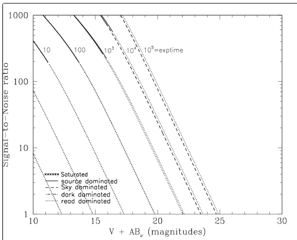
Figure 10.81: Extended source S/N vs. V+AB for the HRC/F660N filter. Top curves are for low sky and bottom curves are for average sky for a 1 arcsec 2 area.
