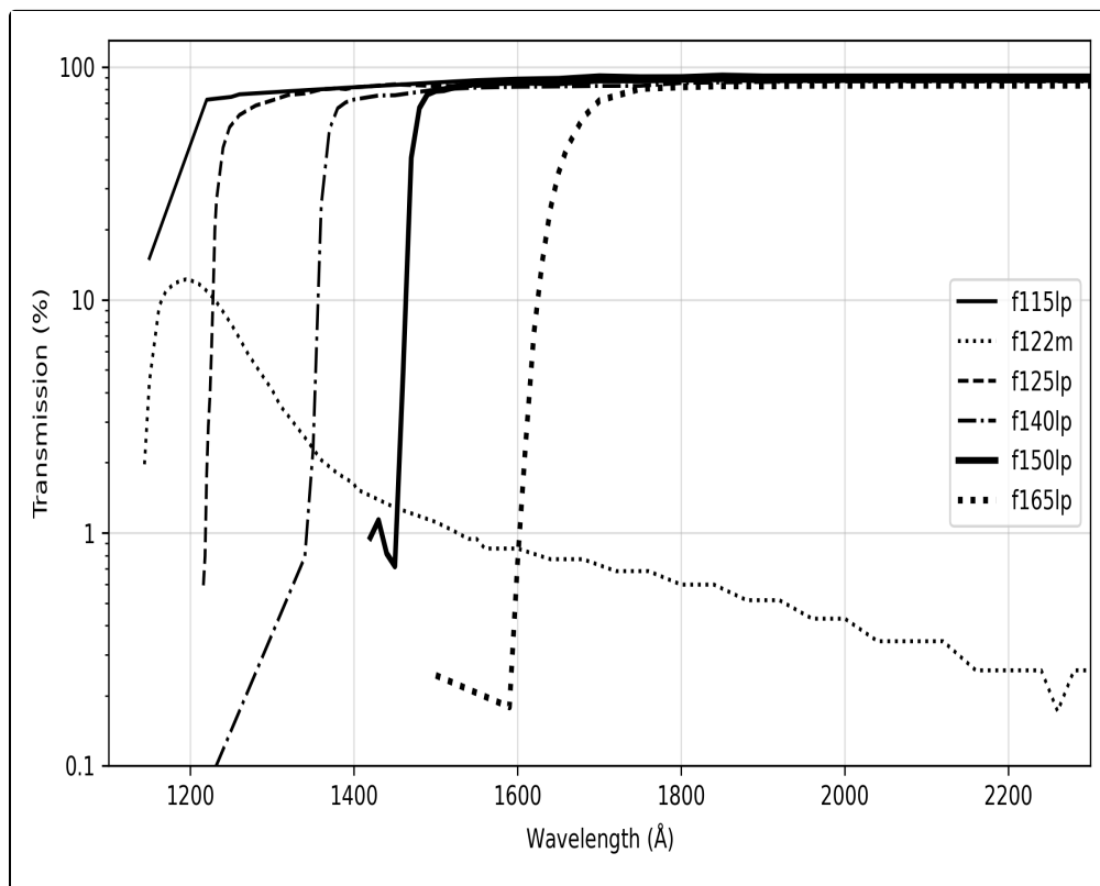
Figure 5.5: ACS SBC filters.
