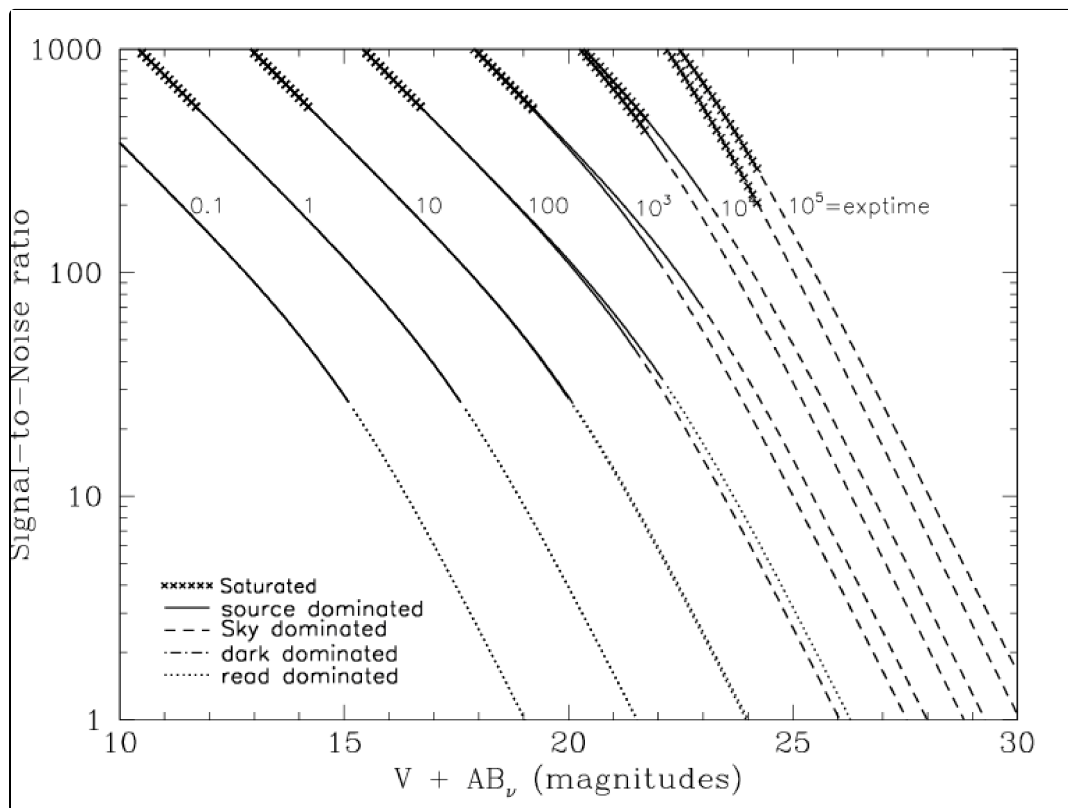
Figure 10.2: Point source S/N vs. V+AB for the WFC/F435W filter. Top curves are for low sky; bottom curves are for average sky.
