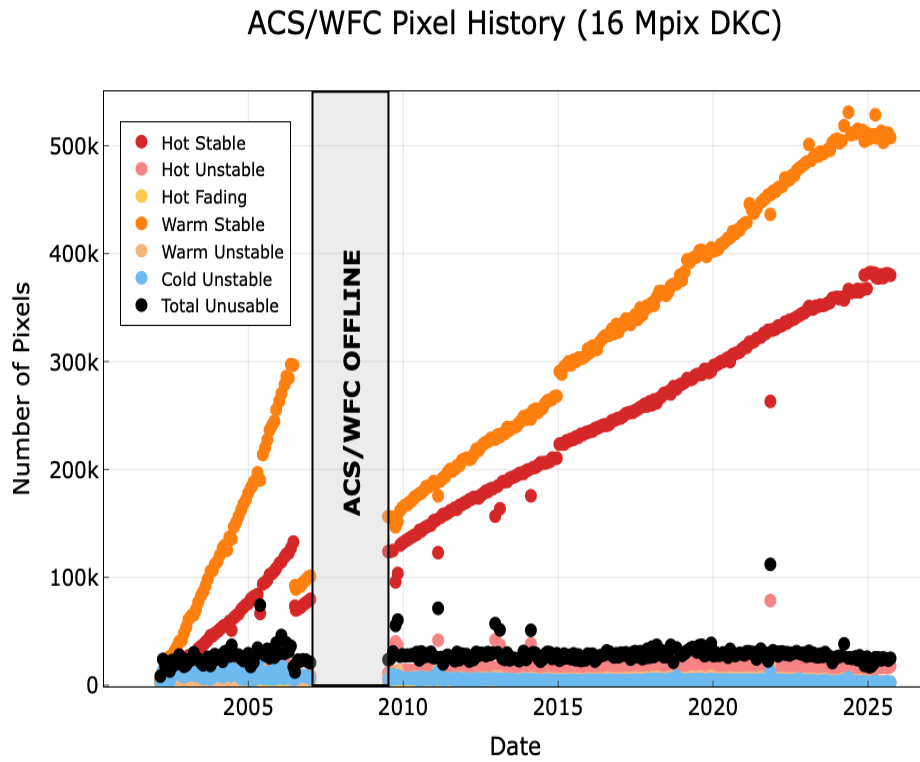
Figure 4.7: Pixel Stability and Hot Pixel Growth in WFC.
