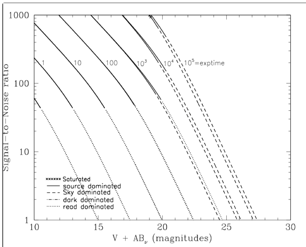
Figure 10.77: Point source S/N vs. V+AB for the HRC/F658N filter. Top curves are for low sky; bottom curves are for average sky.
