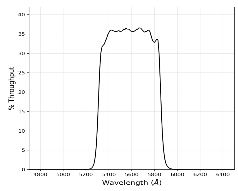
Figure 10.10: Integrated system throughput for WFC/F550M.
