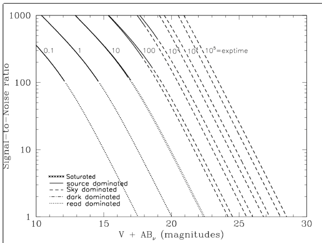
Figure 10.30: Extended source S/N vs. V+AB for the WFC/F775W filter. Top curves are for low sky and bottom curves are for average sky for a 1 \text{ arcsec}^2 area.
