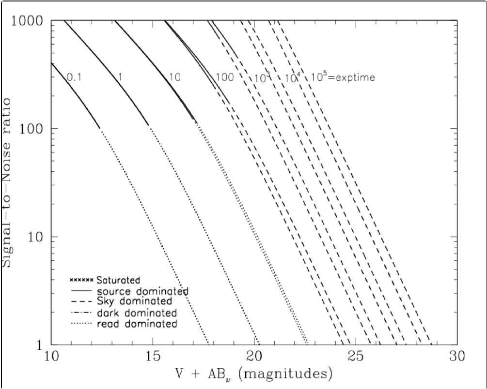
Figure 10.21: Extended source S/N vs. V+AB for the WFC/F625W filter. Top curves are for low sky and bottom curves are for average sky for a 1 arcsec 2 area.
