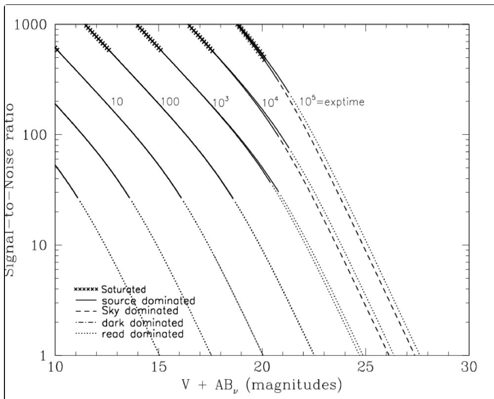
Figure 10.26: Point source S/N vs. V+AB for the WFC/F660N filter. Top curves are for low sky; bottom curves are for average sky.
