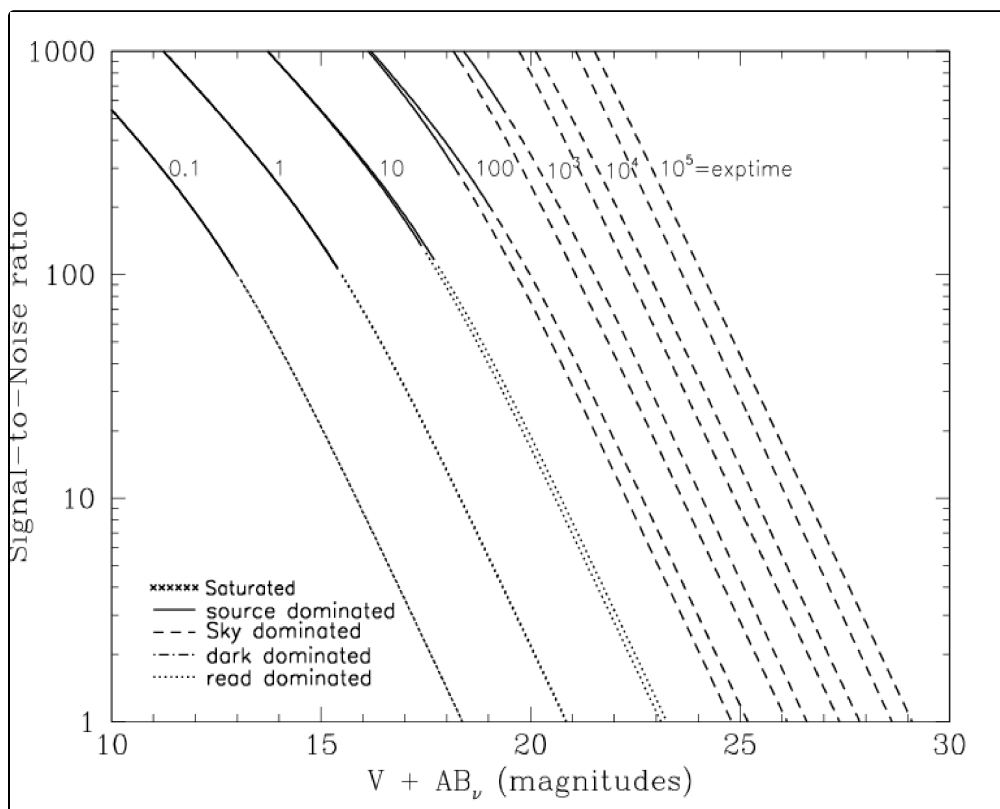
Figure 10.18: Extended source S/N vs. V+AB for the WFC/F606W. Top curves are for low sky and bottom curves are for average sky for a 1 arcsec 2 area.
