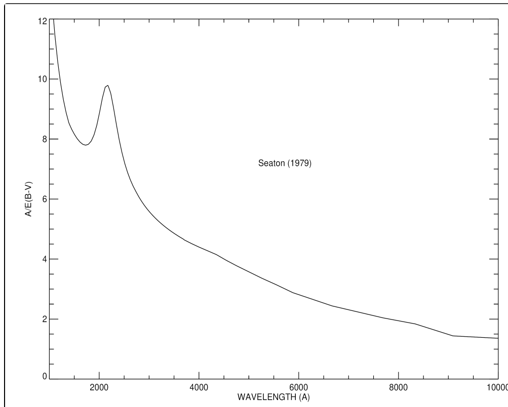
The mean UV interstellar extinction curve of the Milky Way as a function of wavelength. The curve features a prominent bump at 2200 Å, which can disappear at lower metallicities.
