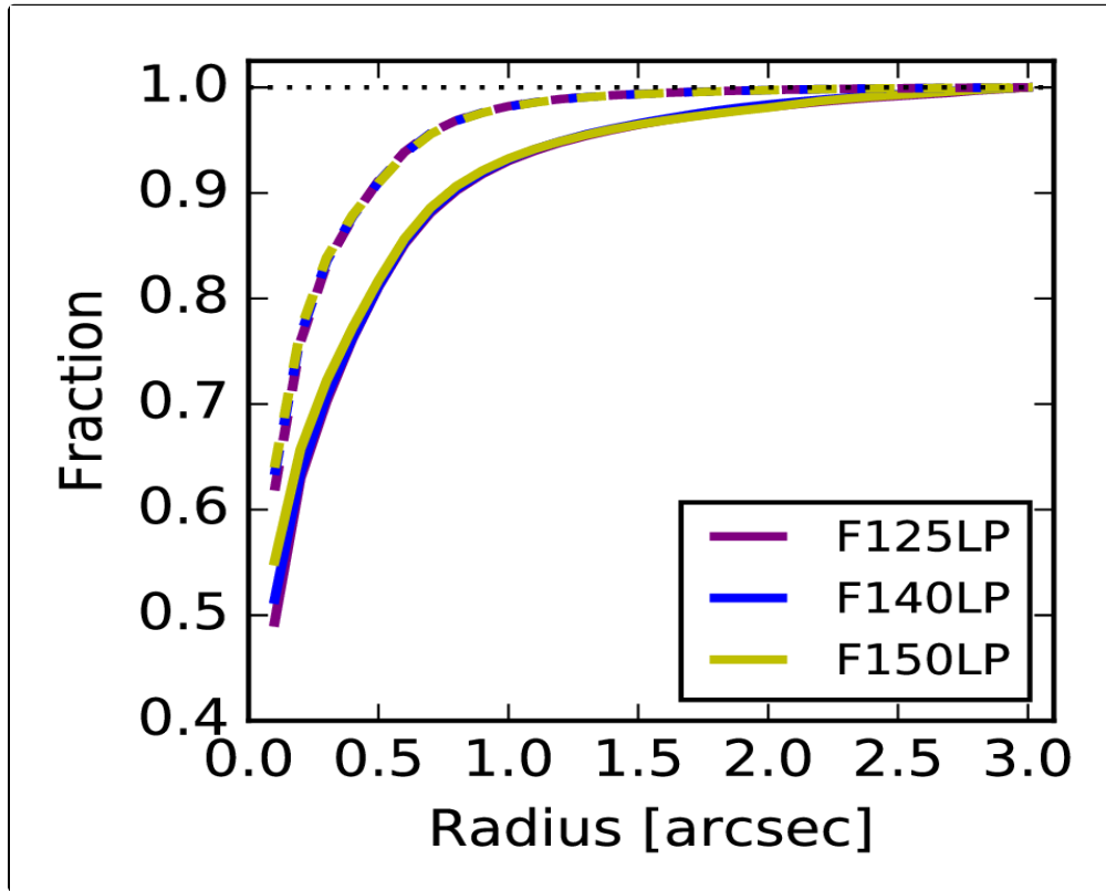
Figure 5.14: Encircled energy for the SBC. Solid lines correspond to observations, dashed lines correspond to Tiny Tim models.
