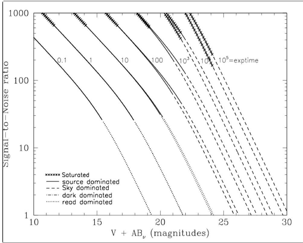
Figure 10.32: Point source S/N vs. V+AB for the WFC/F814W filter. Top curves are for low sky; bottom curves are for average sky.
