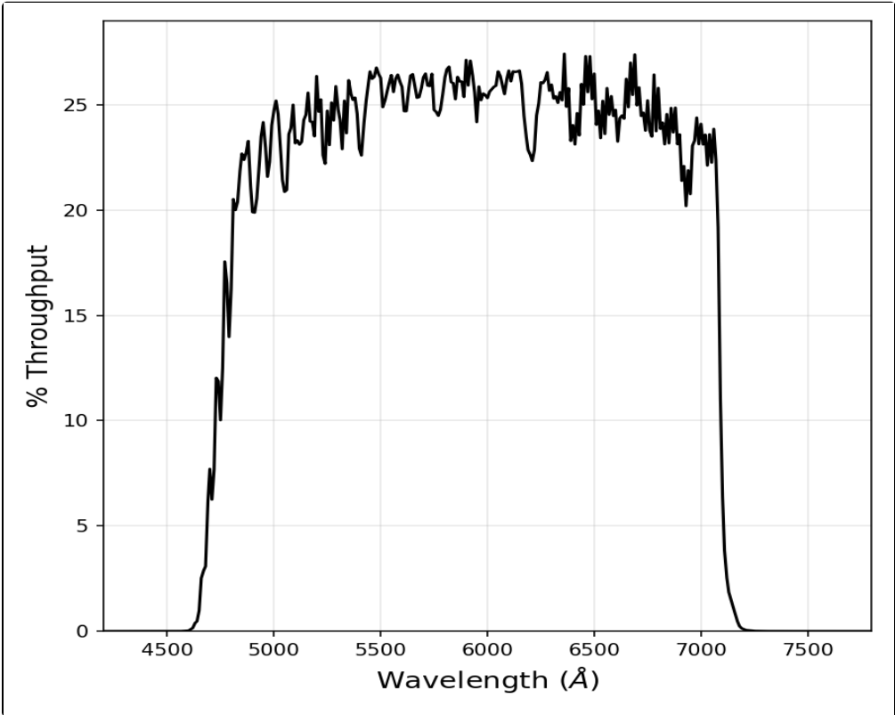
Figure 10.70: Integrated system throughput for HRC/F606W.
