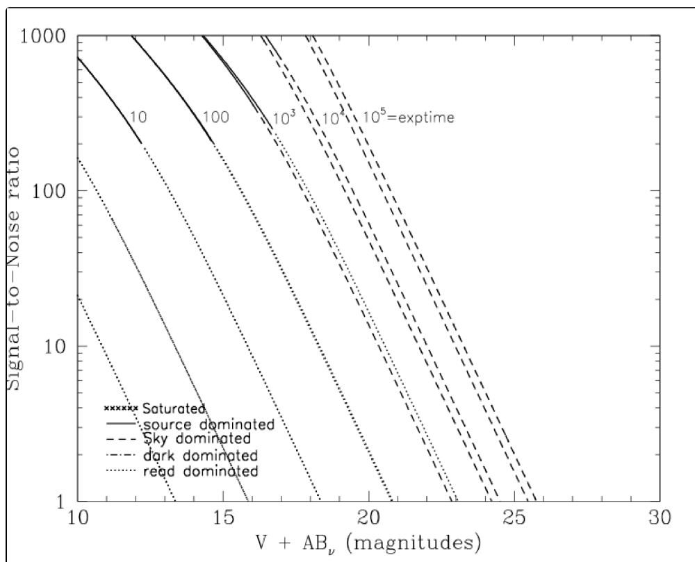
Figure 10.78: Extended source S/N vs. V+AB for the HRC/F658N filter. Top curves are for low sky and bottom curves are for average sky for a 1 arcsec 2 area.
