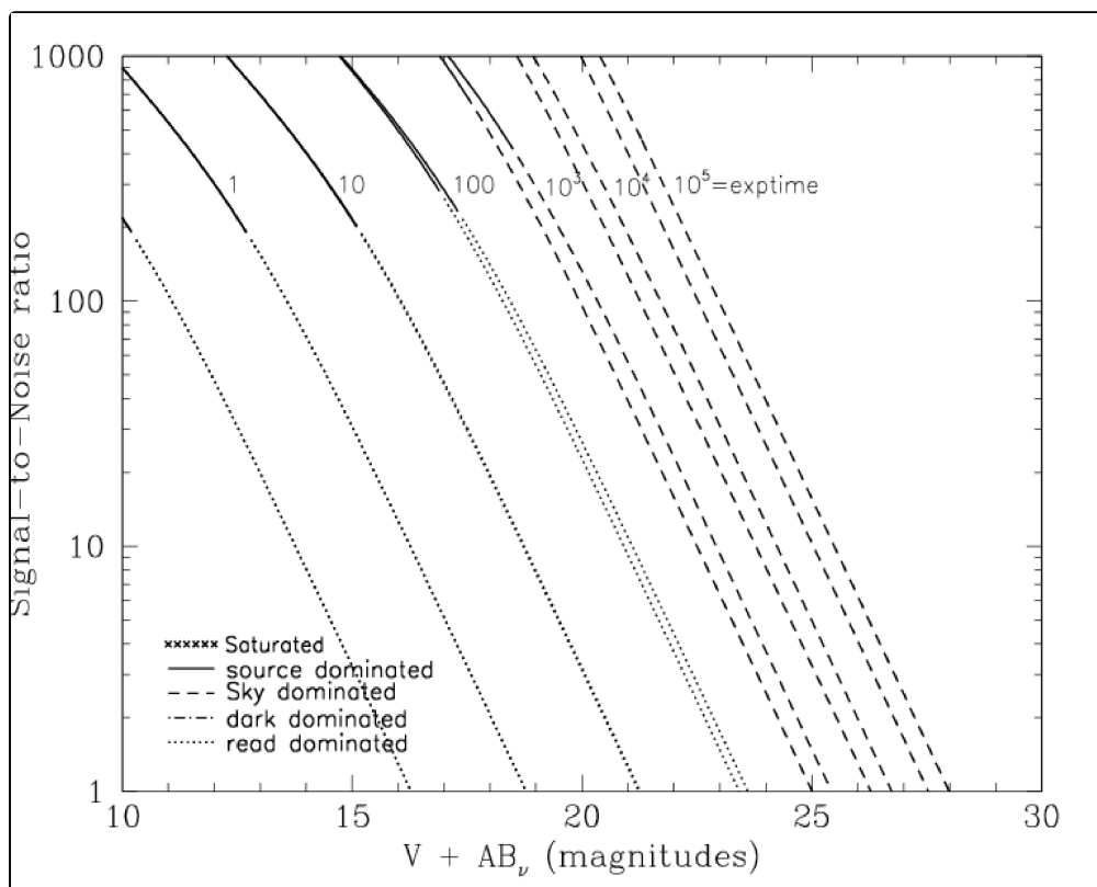
Figure 10.57: Extended source S/N vs. V+AB for the HRC/F435W filter. Top curves are for low sky and bottom curves are for average sky for a 1 arcsec 2 area.
