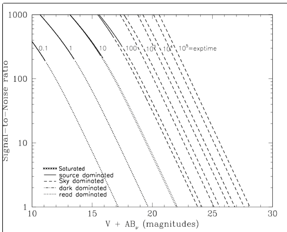
Figure 10.72: Extended source S/N vs. V+AB for the HRC/F606W filter. Top curves are for low sky and bottom curves are for average sky for a 1 arcsec 2 area.
