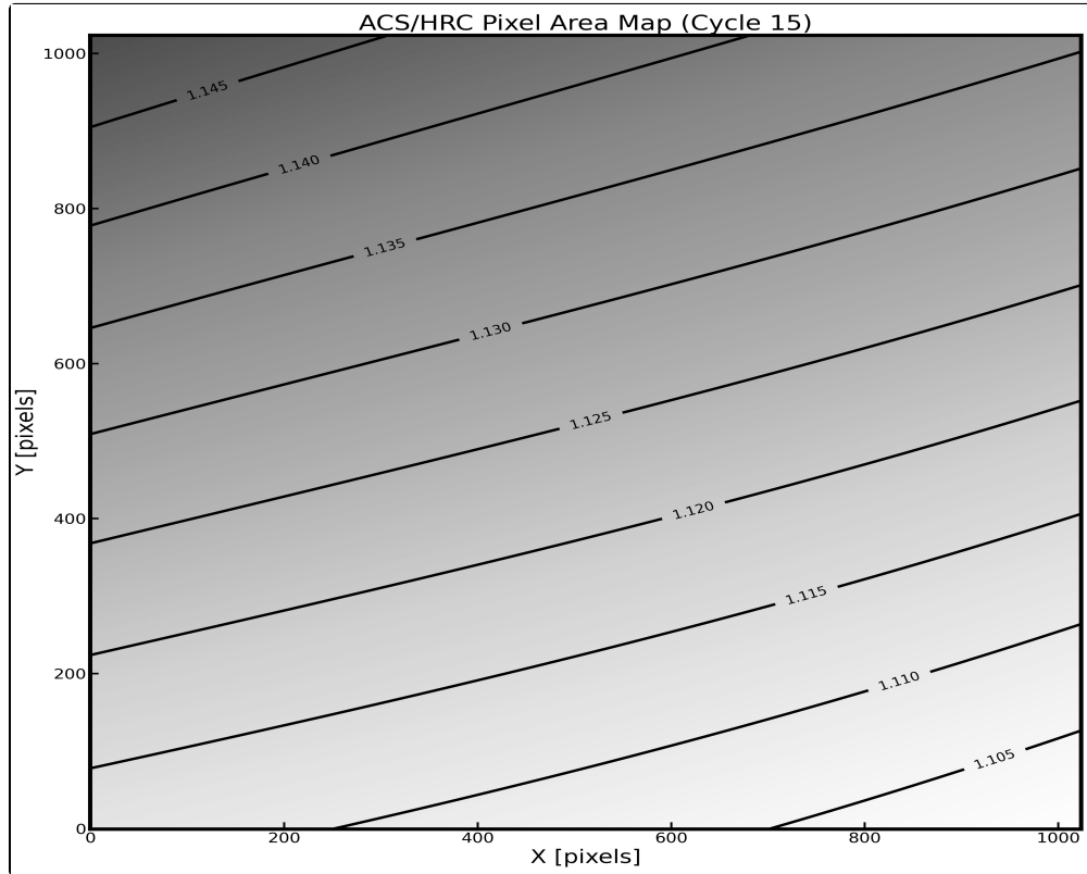
Figure 10.114: Pixel area map of the ACS/HRC chip generated from Cycle 15 data.
