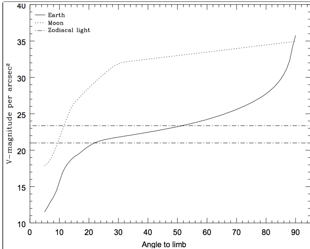
Figure 9.2: Background contributions in V magnitude per arcseconds 2 .
