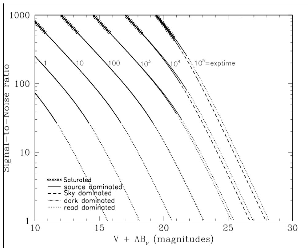
Figure 10.8: Point source S/N vs. V+AB for the WFC/F502N filter. Top curves are for low sky; bottom curves are for average sky.
