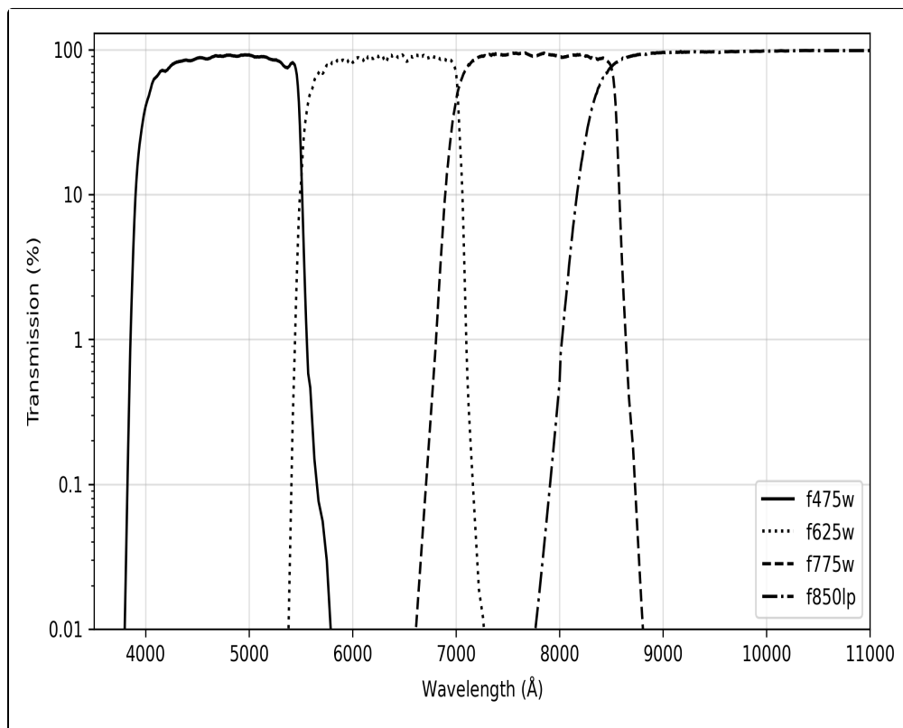
Figure 5.2: ACS SDSS filters.
