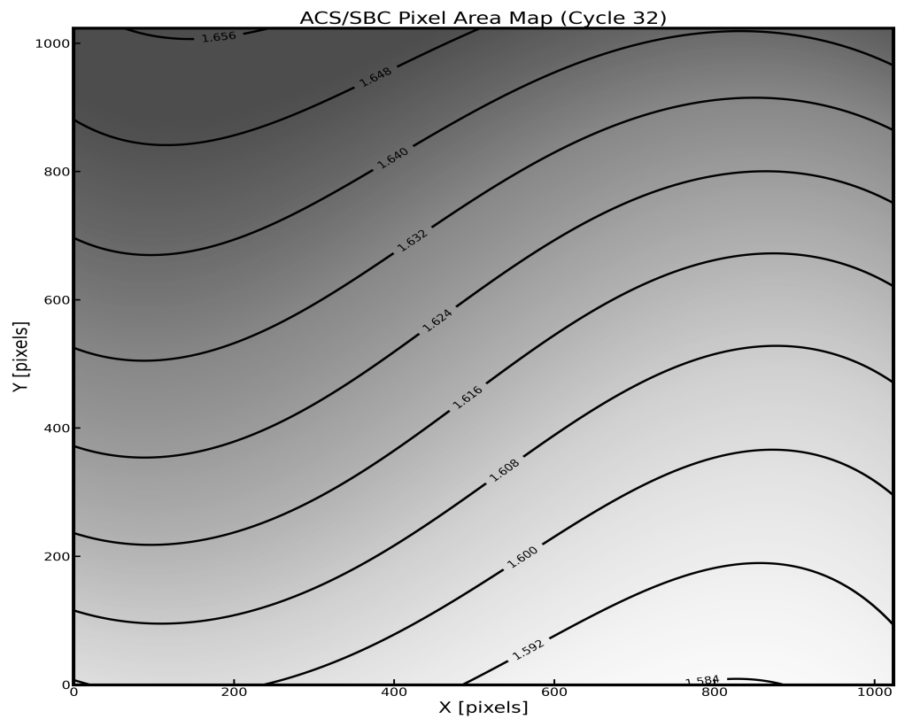
Figure 10.116: The map of the effective pixel areas of the ACS/SBC. The areas are normalized to 0.025 arcsecond square pixels.
