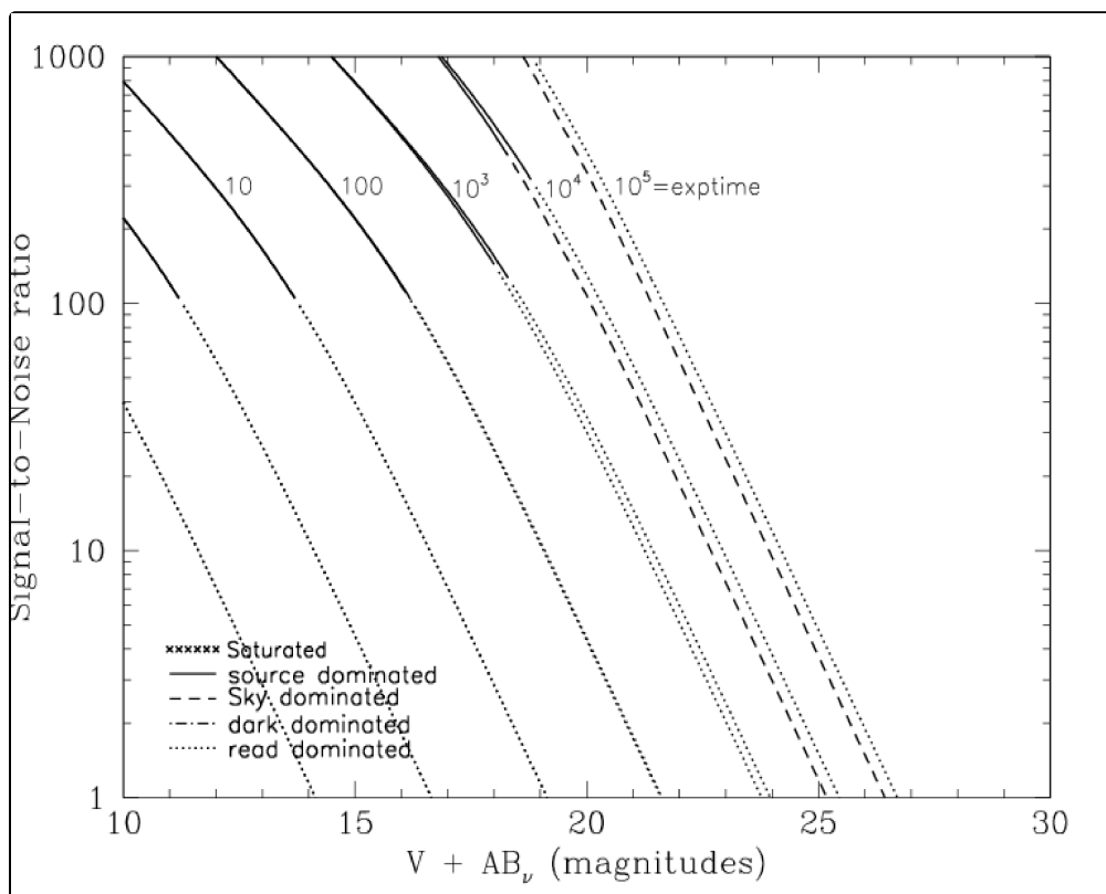
Figure 10.9: Extended source S/N vs. V+AB for the WFC/F502N filter. Top curves are for low sky and bottom curves are for average sky for a 1 arcsec 2 area.
