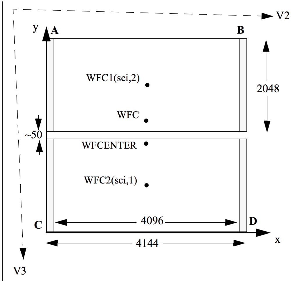
Figure 7.3: WFC full-frame aperture definitions.
