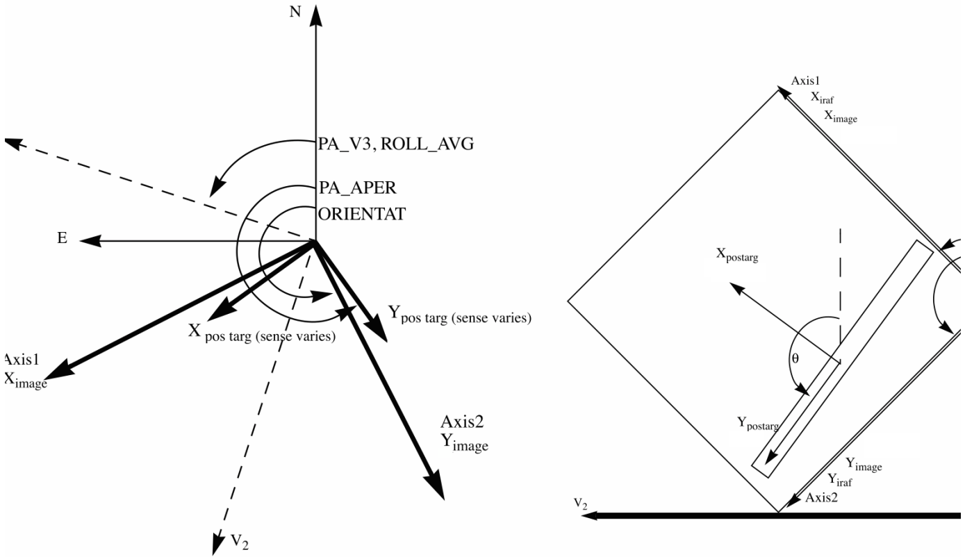
Figure 7.8: Aperture and image feature orientation.
