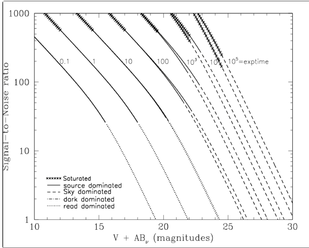
Figure 10.5: Point source S/N vs. V+AB for the WFC/F475W filter. Top curves are for low sky; bottom curves are for average sky.
