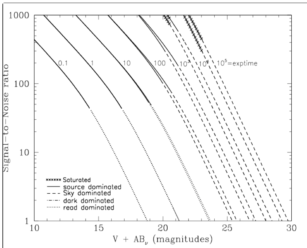
Figure 10.71: Point source S/N vs. V+AB for the HRC/F606W filter. Top curves are for low sky; bottom curves are for average sky.
