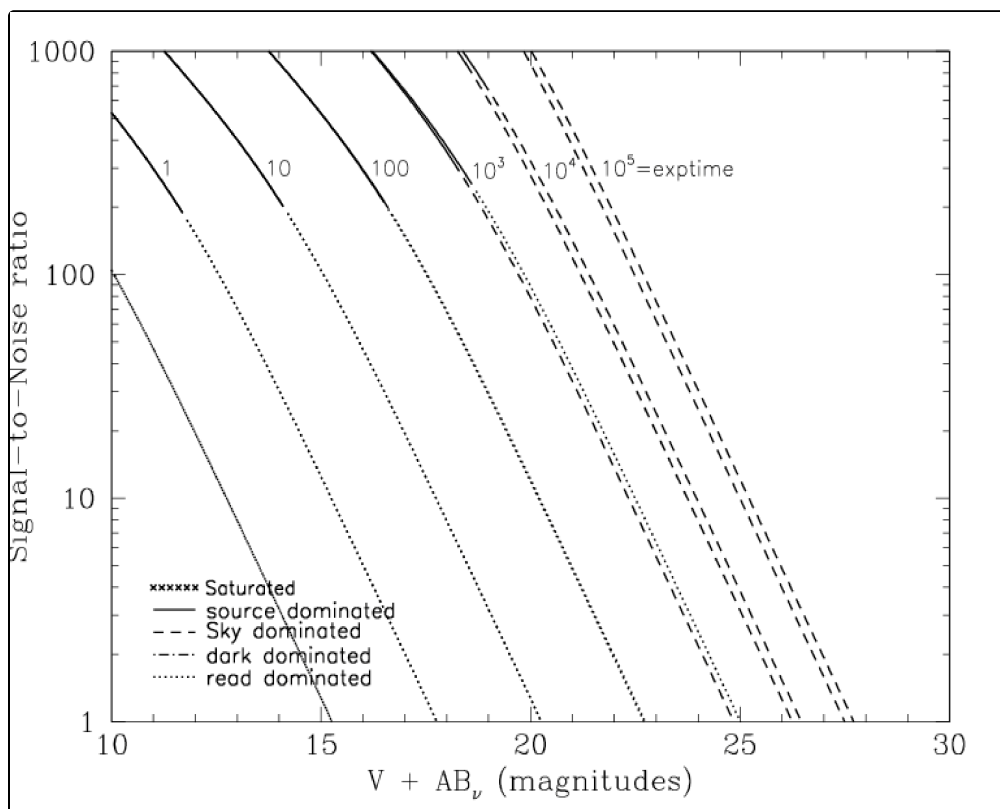
Figure 10.51: Extended source S/N vs. V+AB for the HRC/F330W filter. Top curves are for low sky and bottom curves are for average sky for a 1 arcsec 2 area.
