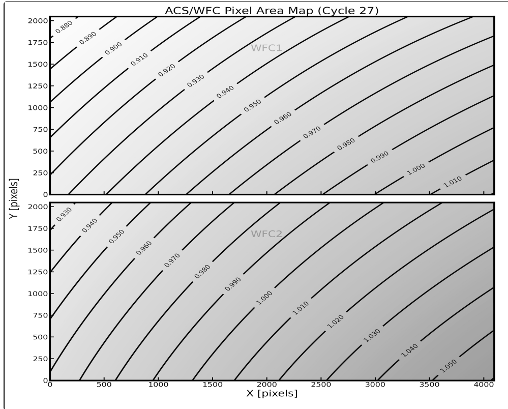
Figure 10.112: Pixel area map of the ACS/WFC chips generated from Cycle 27 data.
