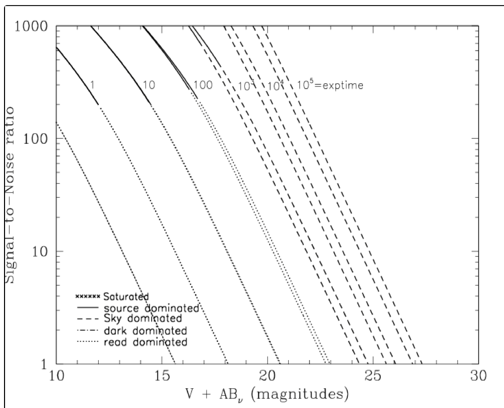
Figure 10.66: Extended source S/N vs. V+AB for the HRC/F550M filter. Top curves are for low sky and bottom curves are for average sky for a 1 arcsec 2 area.
