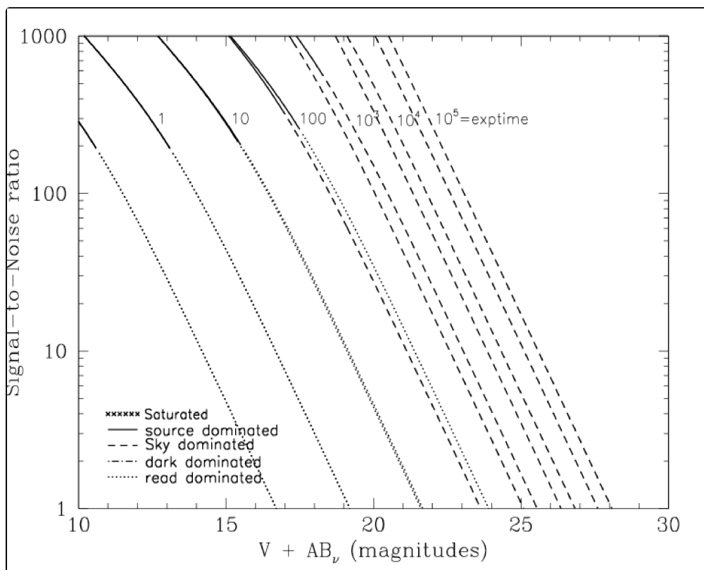
Figure 10.60: Extended source S/N vs. V+AB for the HRC/F475W filter. Top curves are for low sky and bottom curves are for average sky for a 1 \text{ arcsec}^2 area.
