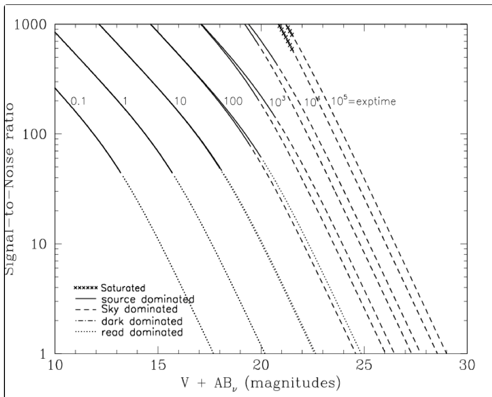
Figure 10.83: Point source S/N vs. V+AB for the HRC/F775W filter. Top curves are for low sky; bottom curves are for average sky.
