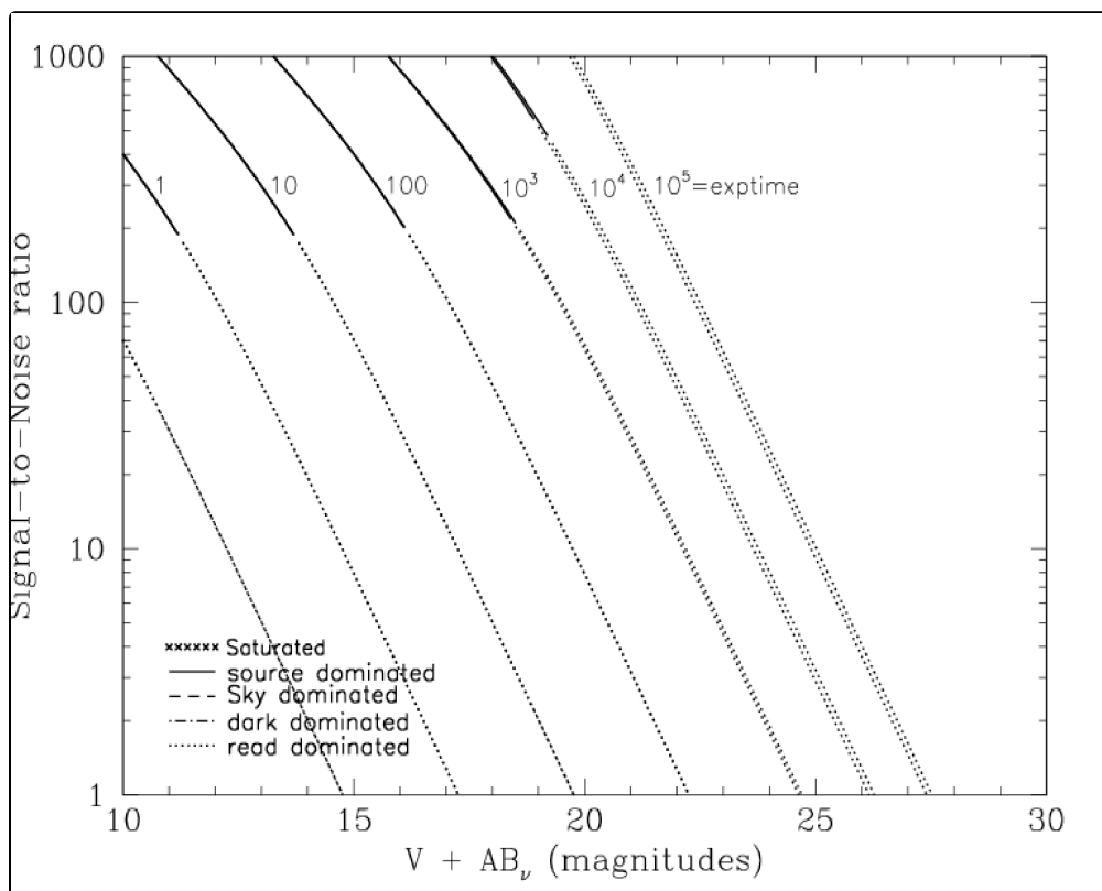
Figure 10.45: Extended source S/N vs. V+AB for the HRC/F220W filter. Top curves are for low sky and bottom curves are for average sky for a 1 \text{ arcsec}^2 area.
