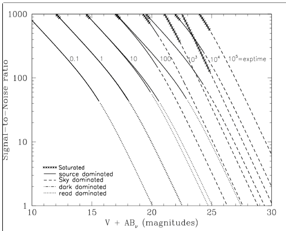
Figure 10.101: Point source S/N vs. V+AB for the HRC/Clear filter. Top curves are for low sky; bottom curves are for average sky.
