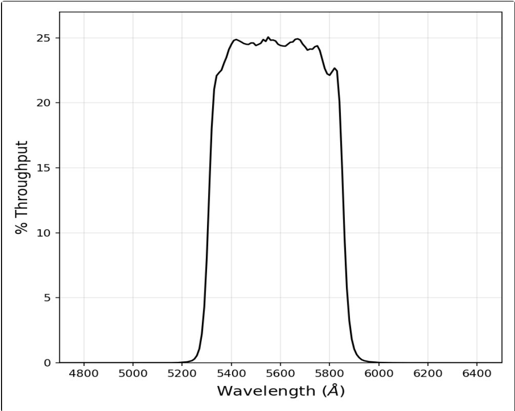
Figure 10.64: Integrated system throughput for HRC/F550M.
