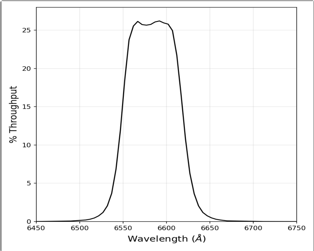
Figure 10.76: Integrated system throughput for HRC/F658N.
