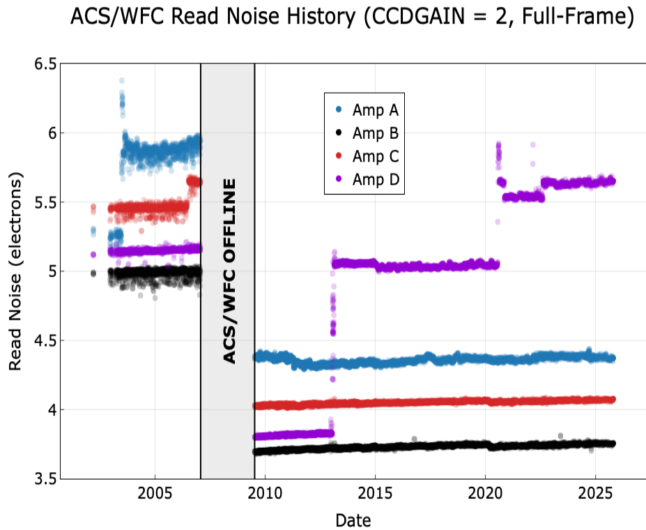
Figure 4.6: History of ACS/WFC read noise
