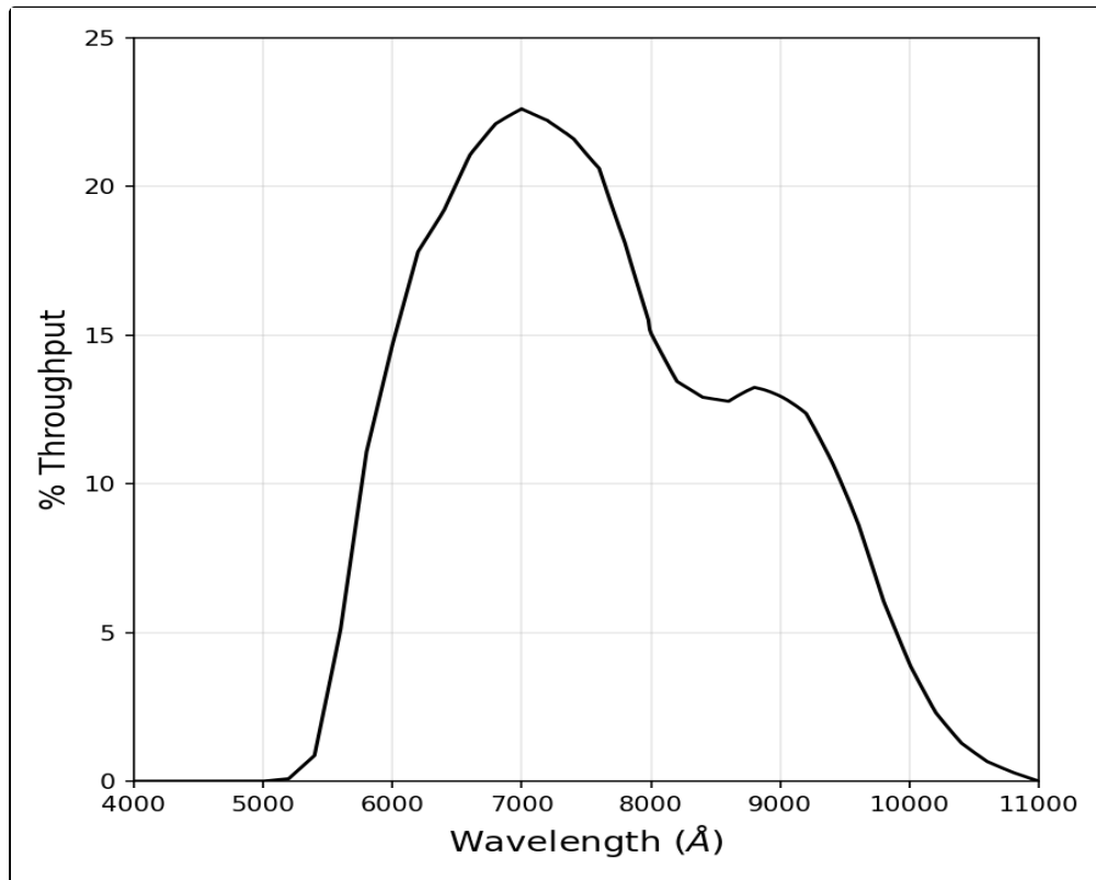
Figure 10.94: Integrated system throughput for HRC/G800L.
