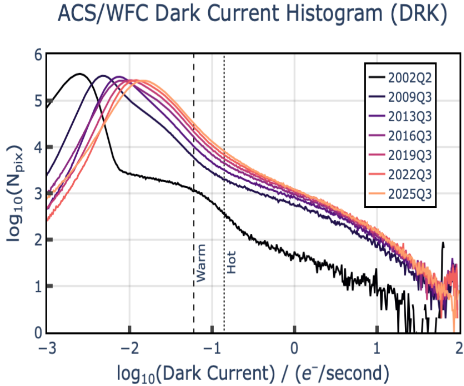
Figure 4.9: ACS/WFC Dark Current Histograms
