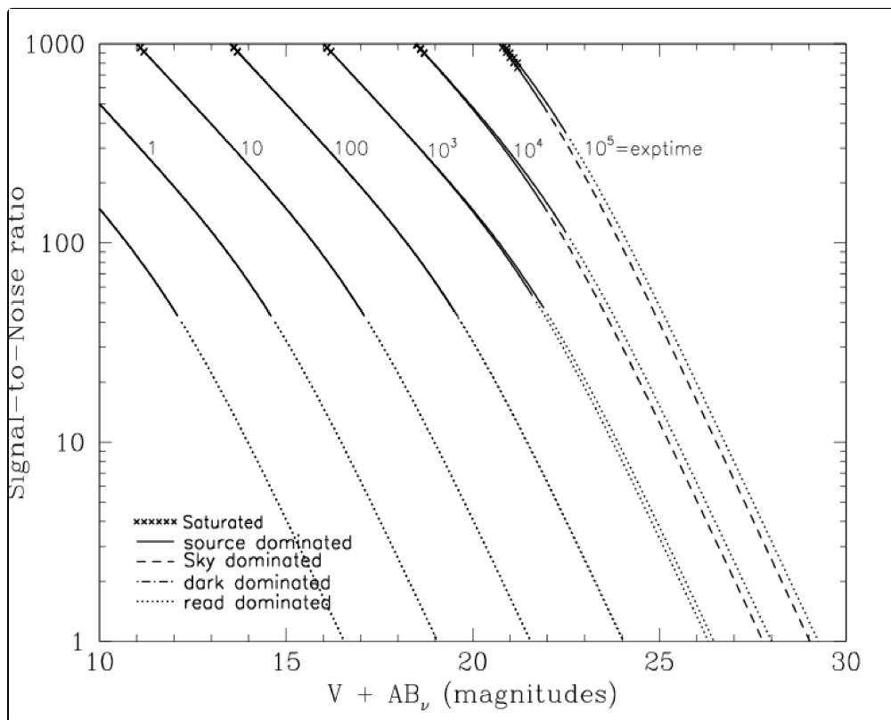
Figure 10.47: Point Source S/N vs. V+AB for the HRC/F250W filter. Top curves are for low sky; bottom curves are for average sky.
