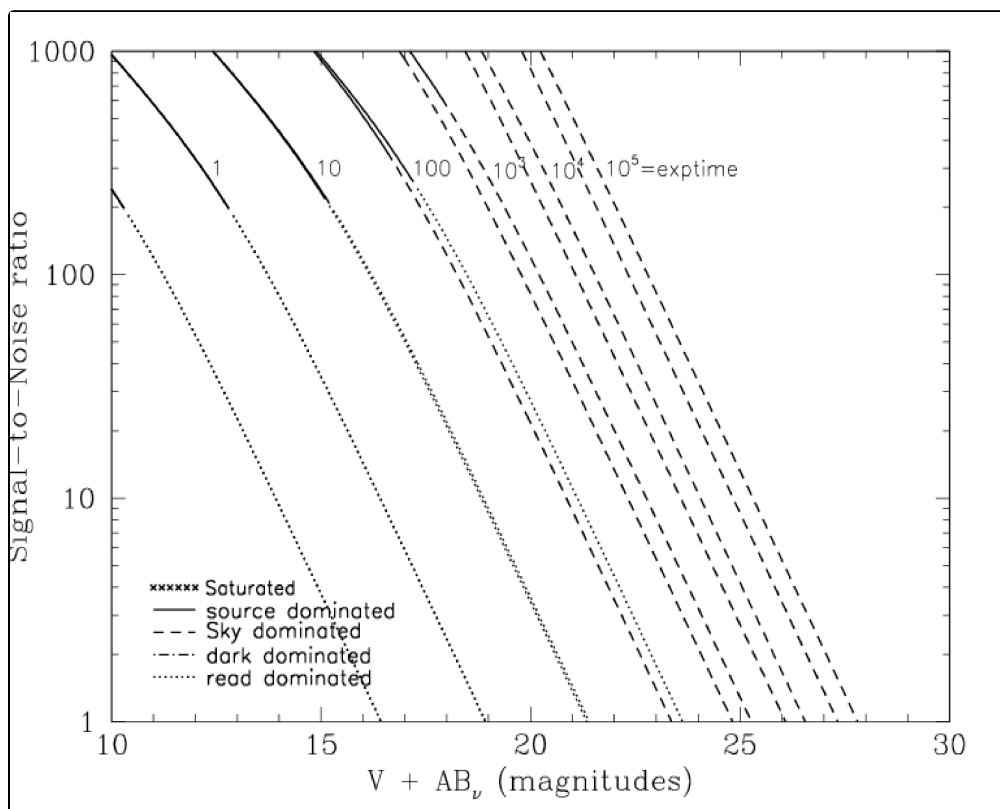
Figure 10.69: Extended source S/N vs. V+AB for the HRC/F555W filter. Top curves are for low sky and bottom curves are for average sky for a 1 arcsec 2 area.
