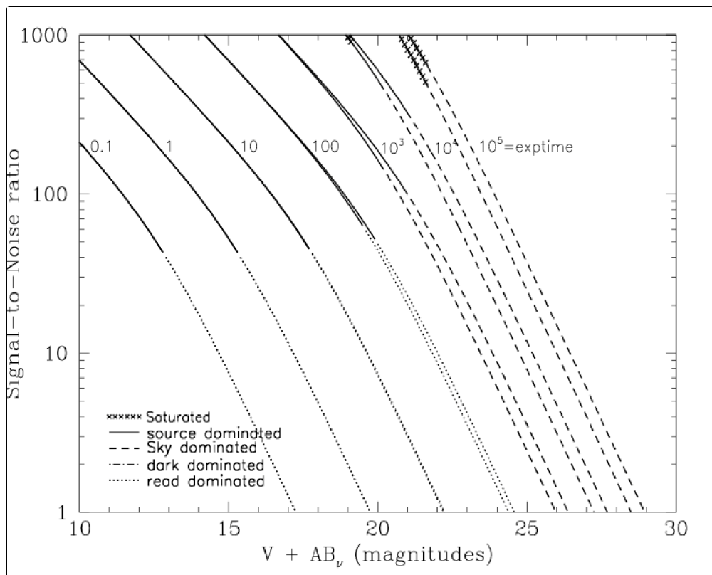
Figure 10.65: Point source S/N vs. V+AB for the HRC/F550M filter. Top curves are for low sky; bottom curves are for average sky.
