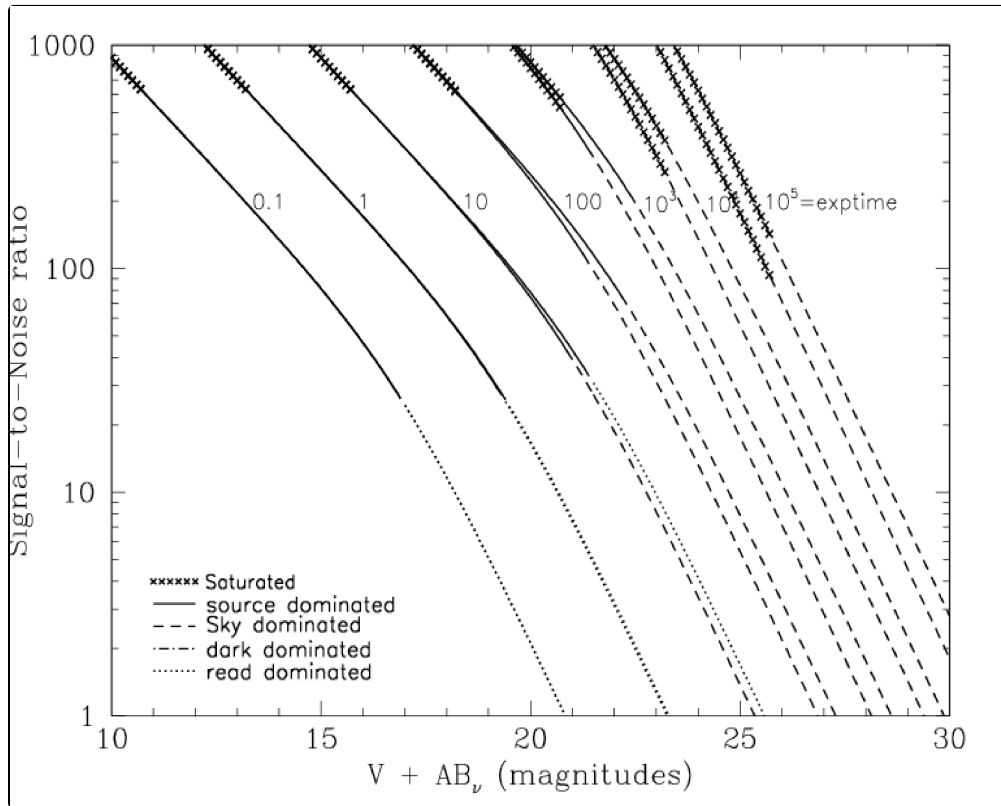
Figure 10.41: Point source S/N vs. V+AB for the WFC/Clear filter. Top curves are for low sky; bottom curves are for average sky.
