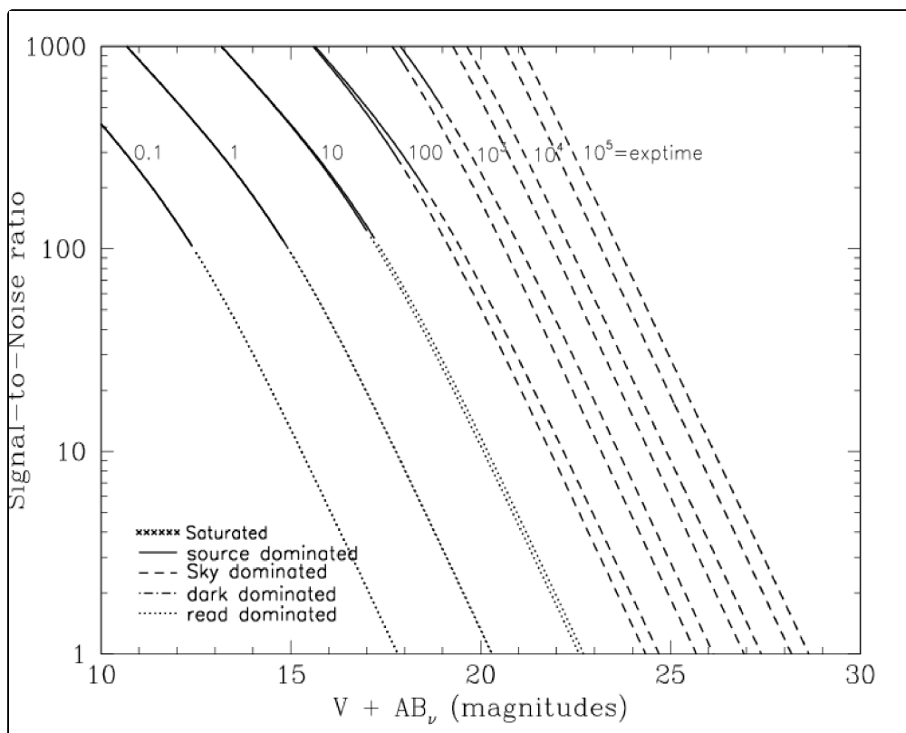
Figure 10.33: Extended source S/N vs. V+AB for the WFC/F814W filter. Top curves are for low sky and bottom curves are for average sky for a 1 arcsec 2 area.
