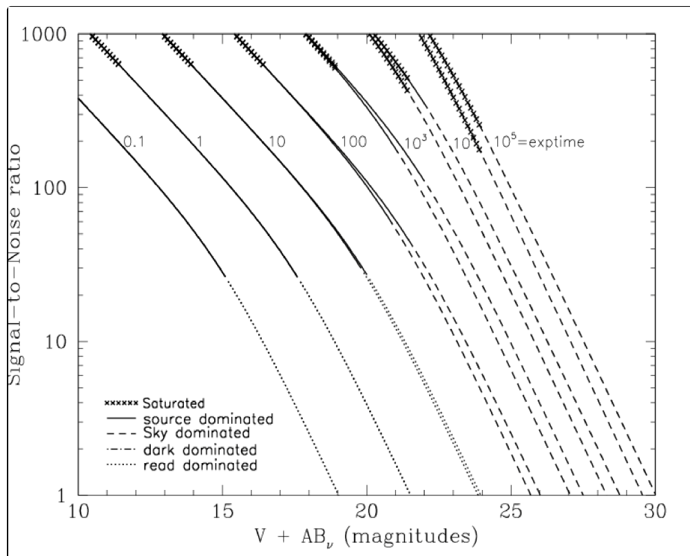
Figure 10.29: Point source S/N vs. V+AB for the WFC/F775W filter. Top curves are for low sky; bottom curves are for average sky.
