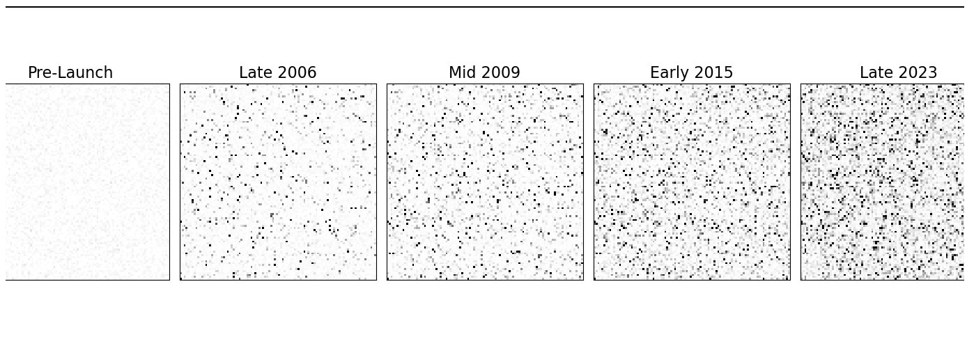
Figure 4.10: A subsection of WFC1 dark frames taken at different epochs showing the increasing population of hot pixels. From left to right: before launch, late 2006 (4 years on orbit), mid 2009 (7 years on orbit), early 2015 (12 years on orbit), and late 2023 (21 years on orbit).
