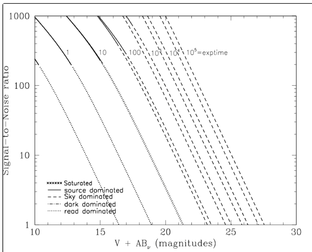
Figure 10.87: Extended source S/N vs. V+AB for the HRC/F814W filter. Top curves are for low sky and bottom curves are for average sky for a 1 arcsec 2 area.
