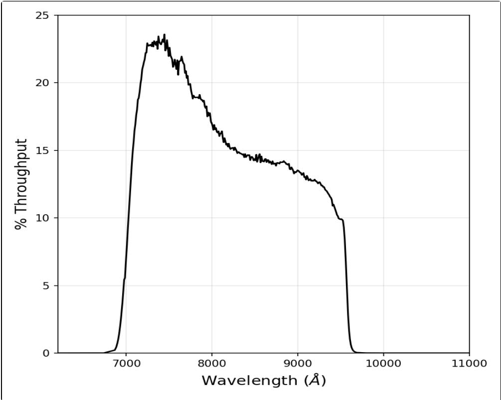
Figure 10.85: Integrated system throughput for HRC/F814W.
