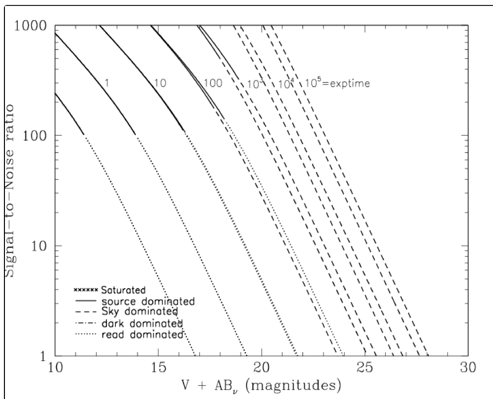
Figure 10.36: Extended source S/N vs. V+AB for the WFC/F850LP filter. Top curves are for low sky and bottom curves are for average sky for a 1 arcsec 2 area.
