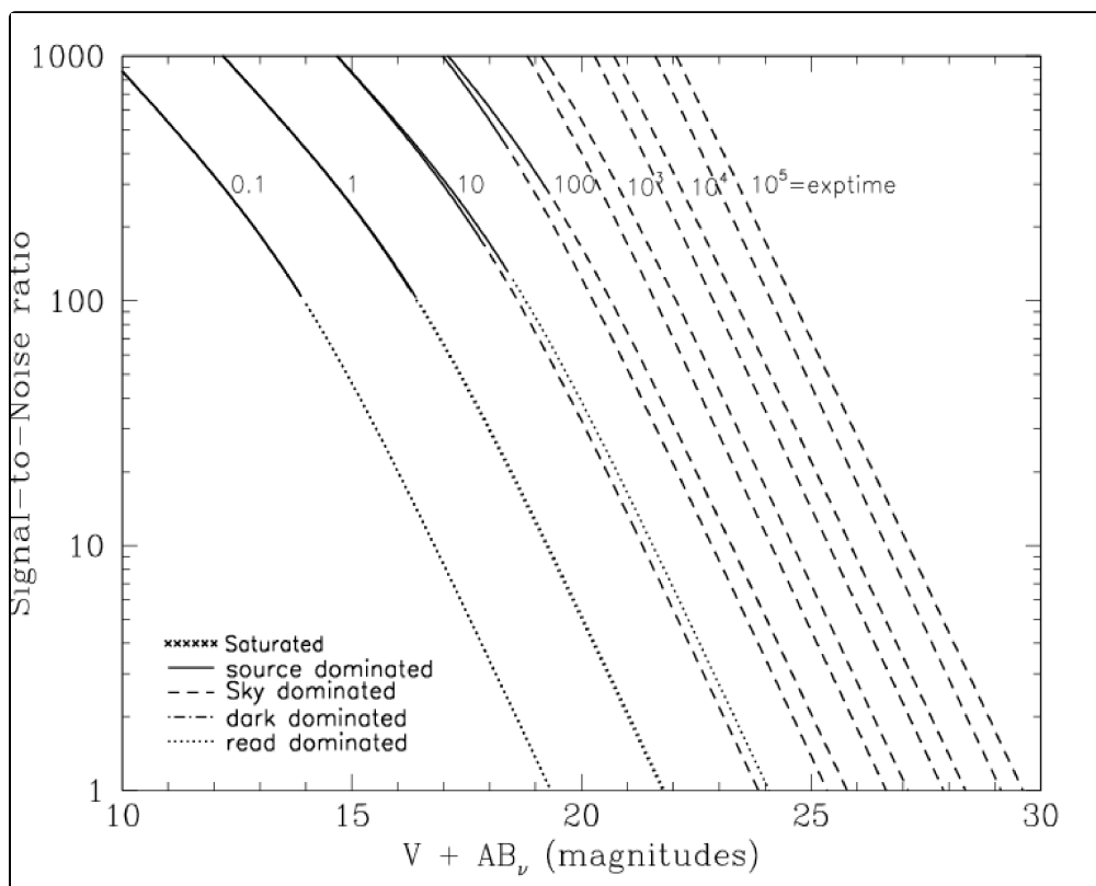
Figure 10.42: Extended source S/N vs. V+AB for the WFC/Clear filter. Top curves are for low sky and bottom curves are for average sky for a 1 arcsec 2 area.
