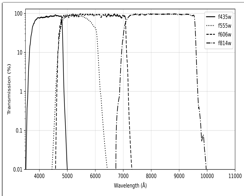
Figure 5.1: ACS broad-band filters.
