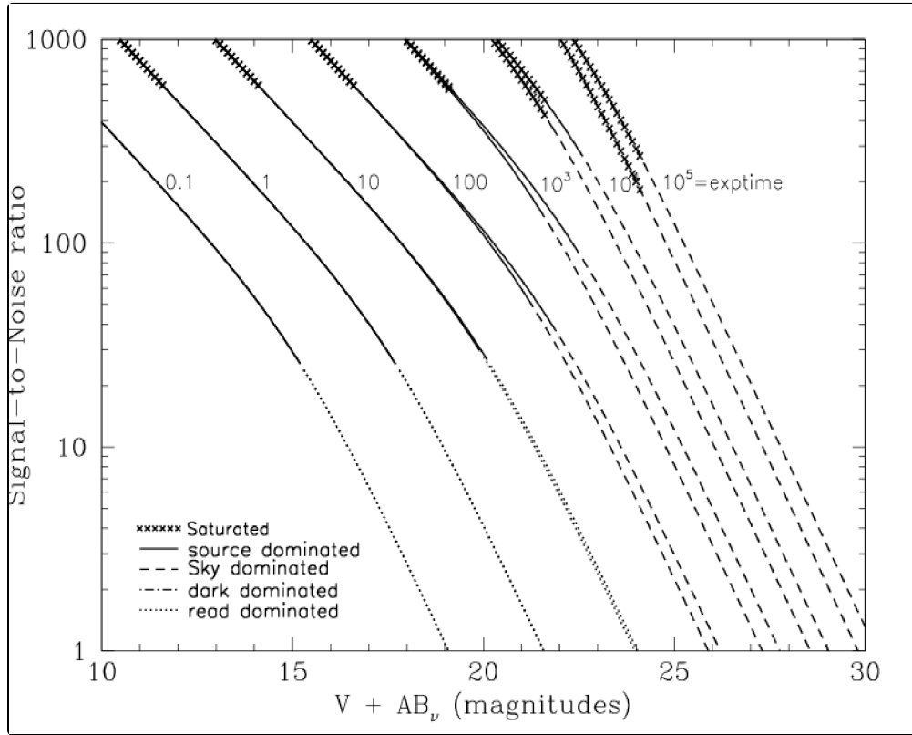
Figure 10.14: Point source S/N vs. V+AB for the WFC/F555W filter. Top curves are for low sky; bottom curves are for average sky.
