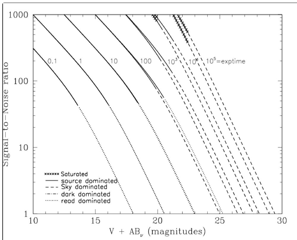
Figure 10.68: Point source S/N vs. V+AB for the HRC/F555W filter. Top curves are for low sky; bottom curves are for average sky.
