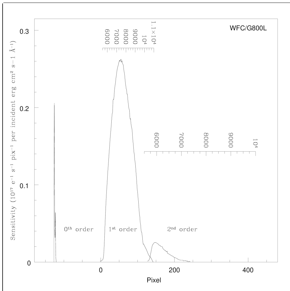
Figure 6.17: Fully dispersed spectrum for white dwarf GD153 with WFC/G800L.
