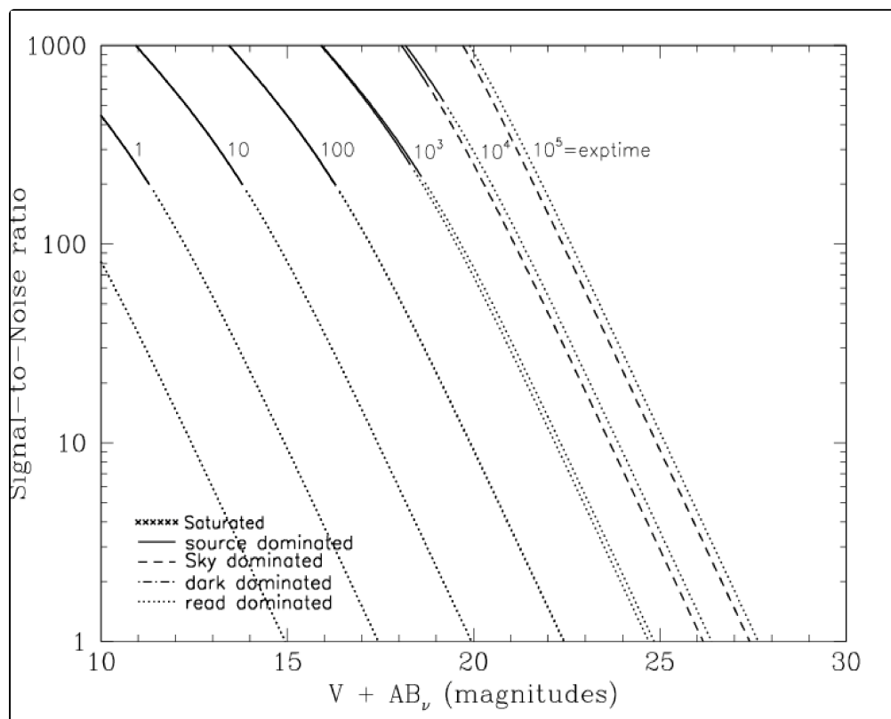
Figure 10.48: Extended Source S/N vs. V+AB for the HRC/F250W filter. Top curves are for low sky and bottom curves are for average sky for a 1 arcsec 2 area.
