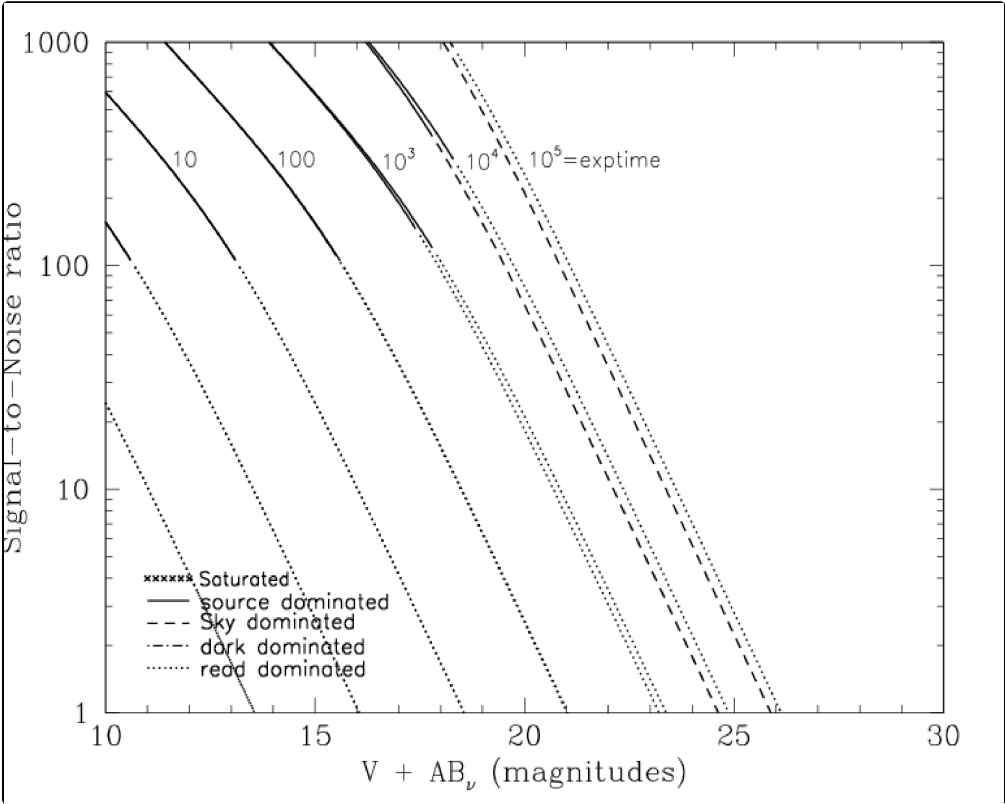
Figure 10.27: Extended source S/N vs. V+AB for the WFC/F660N filter. Top curves are for low sky and bottom curves are for average sky for a 1 arcsec 2 area.
