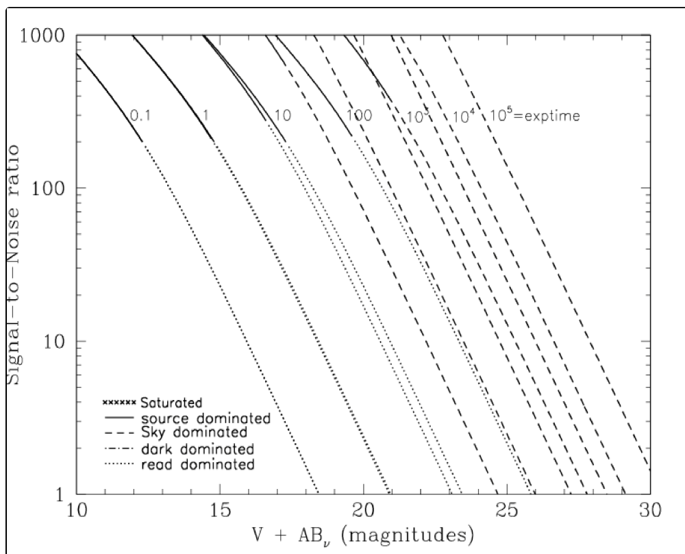
Figure 10.102: Extended source S/N vs. V+AB for the HRC/Clear filter. Top curves are for low sky and bottom curves are for average sky for a 1 arcsec 2 area.
