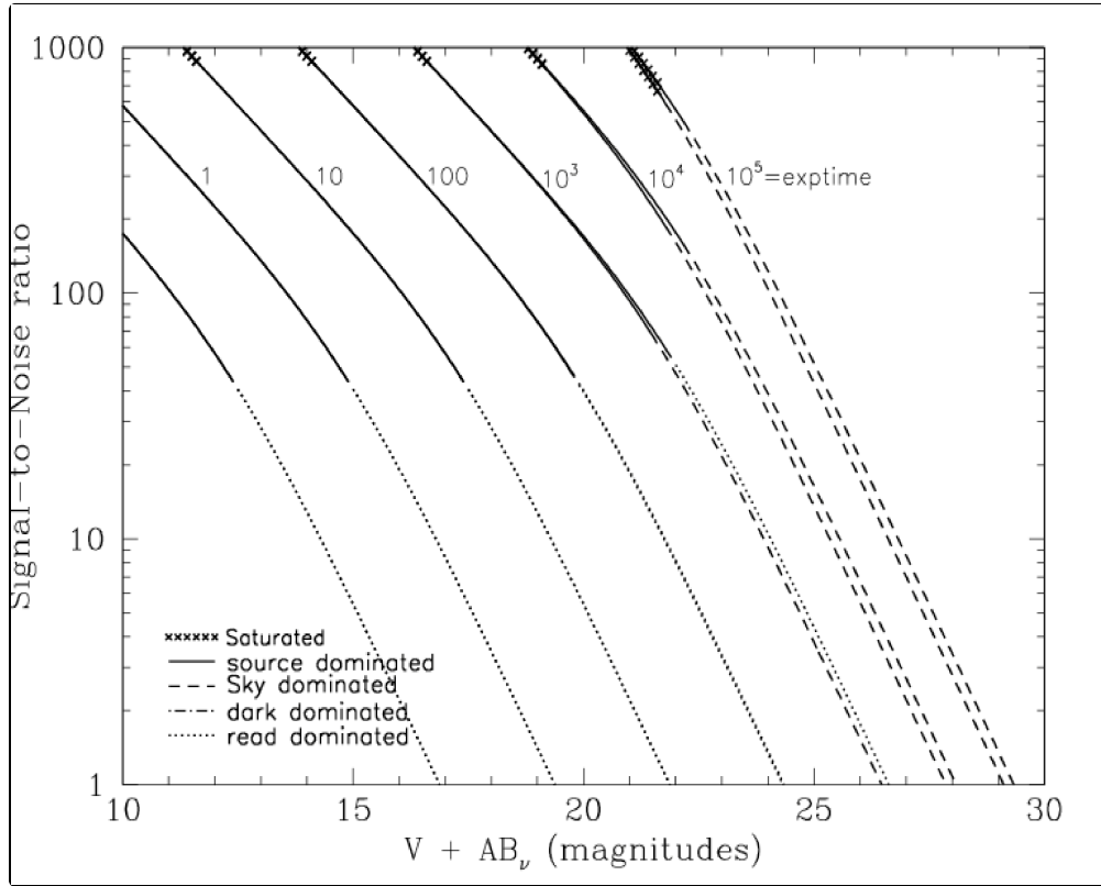
Figure 10.50: Point source S/N vs. V+AB for the HRC/F330W filter. Top curves are for low sky; bottom curves are for average sky.
