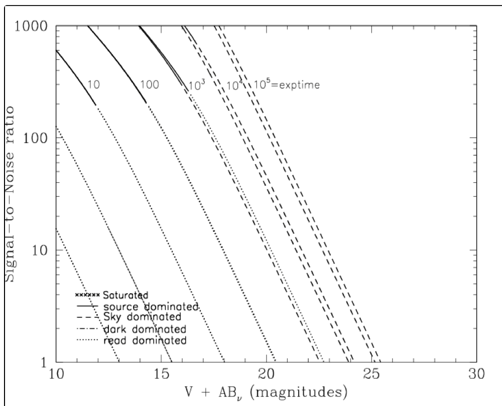
Figure 10.93: Extended source S/N vs. V+AB for the HRC/F892N filter. Top curves are for low sky and bottom curves are for average sky for a 1 arcsec 2 area.
