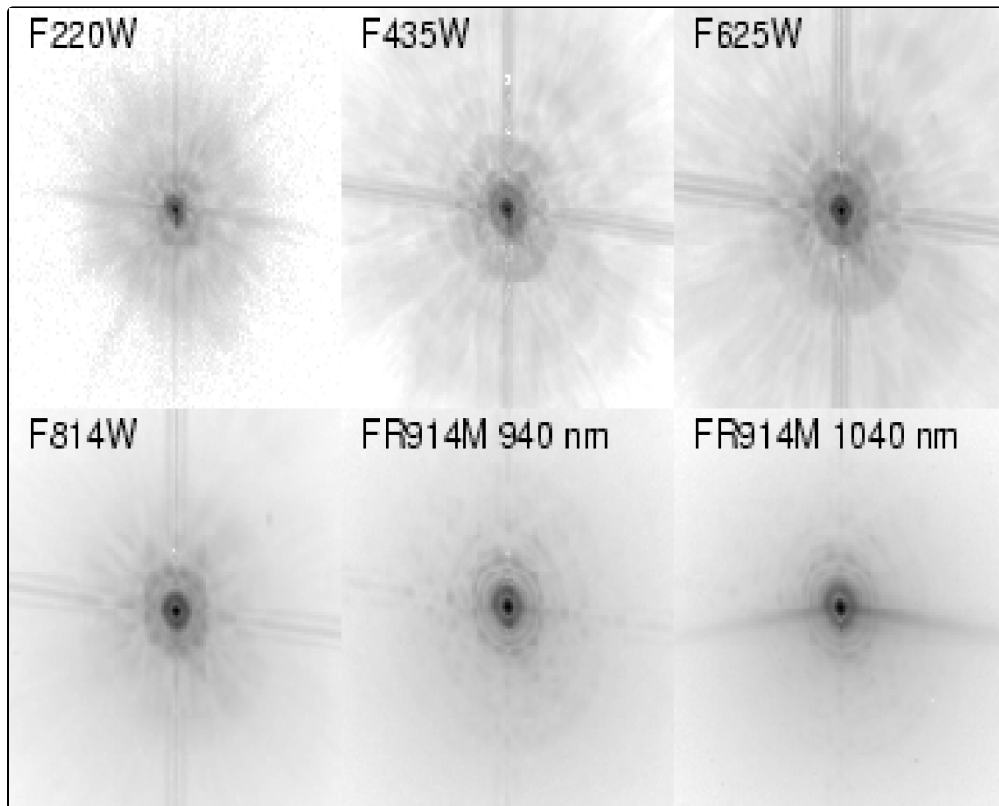
Figure 5.18: ACS HRC PSFs ( 3.25 \times 3.25 arcsec 2 ).
