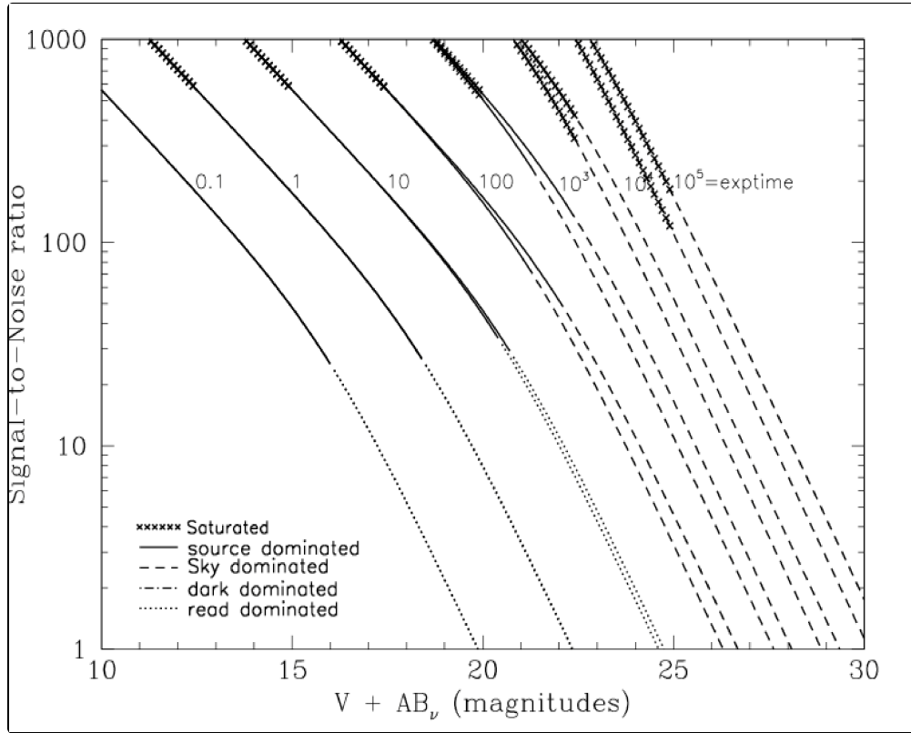
Figure 10.17: Point source S/N vs. V+AB for the WFC/F606W filter. Top curves are for low sky; bottom curves are for average sky.
