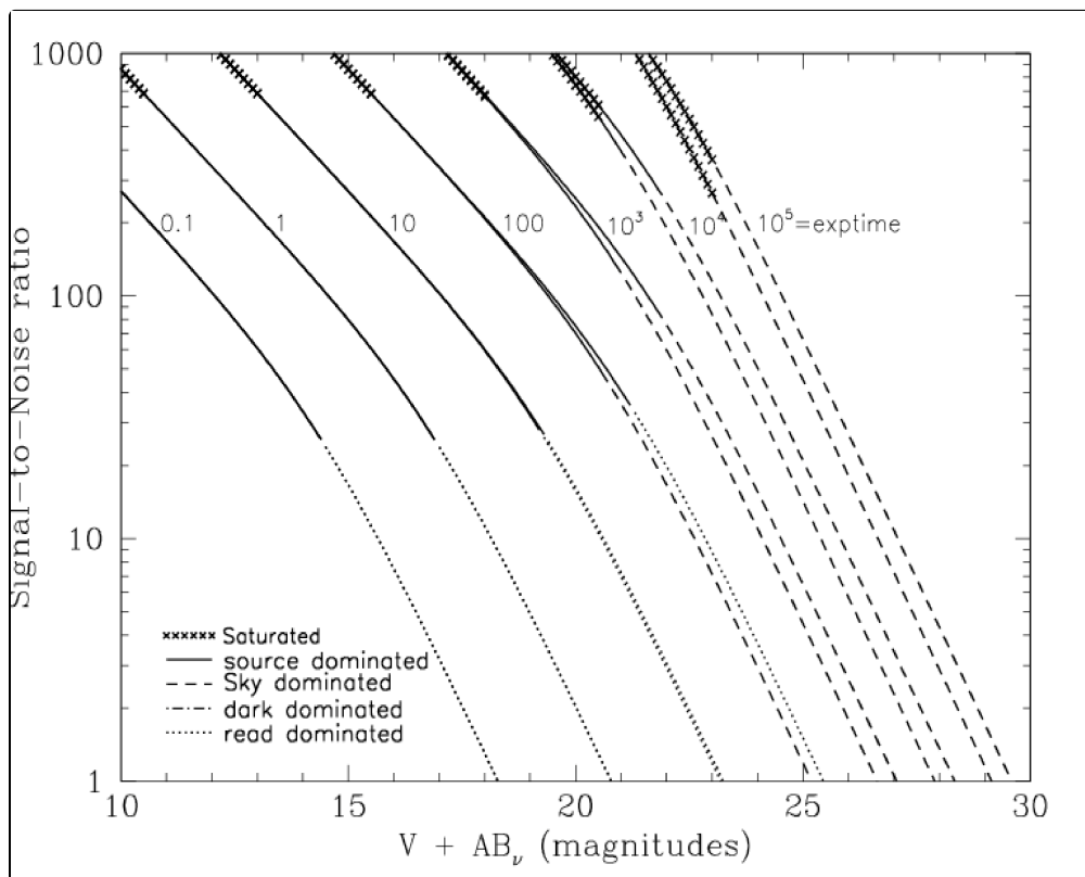
Figure 10.35: Point source S/N vs. V+AB for the WFC/F850LP filter. Top curves are for low sky; bottom curves are for average sky.
