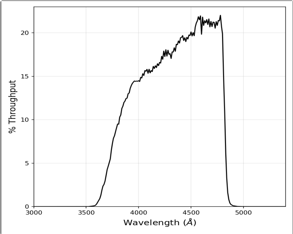
Figure 10.55: Integrated system throughput for HRC/F435W.
