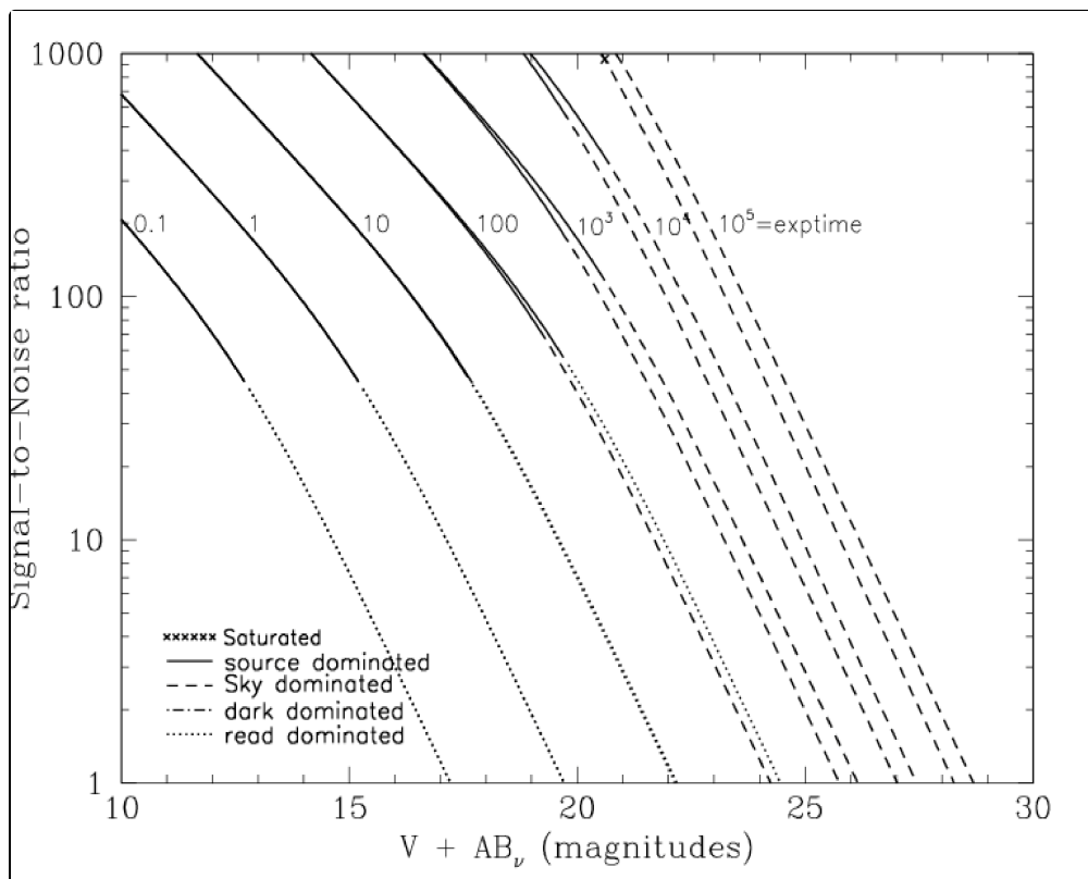
Figure 10.89: Point source S/N vs. V+AB for the HRC/F850LP filter. Top curves are for low sky; bottom curves are for average sky.
