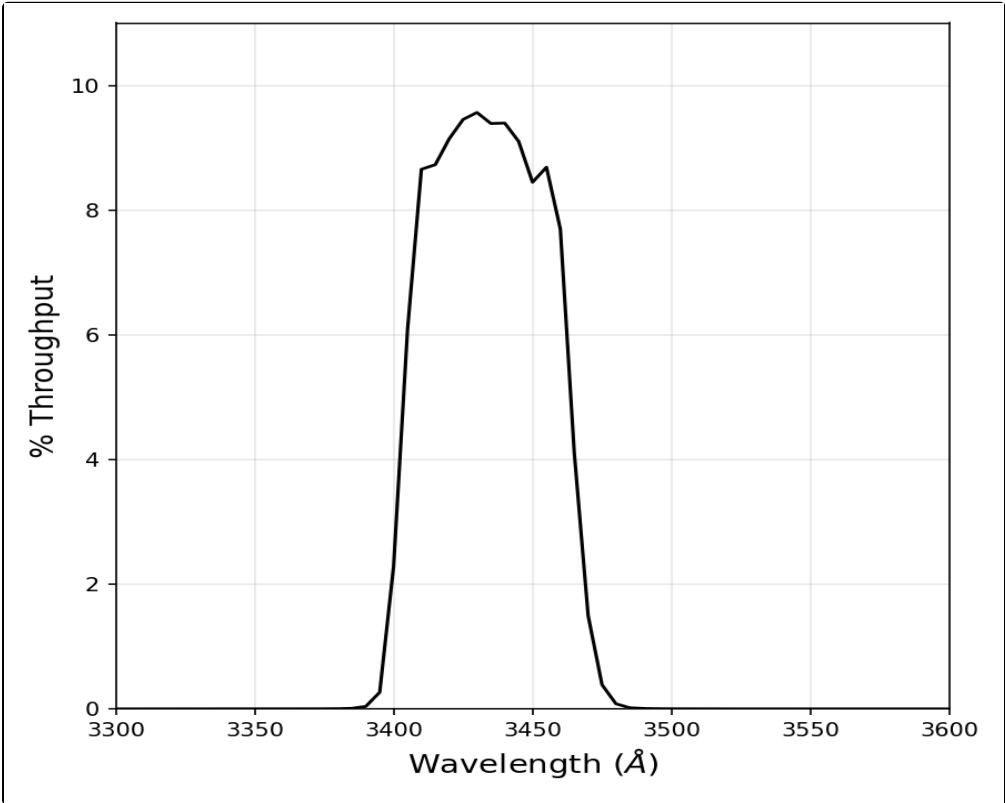
Figure 10.52: Integrated system throughput for HRC/F344N.
