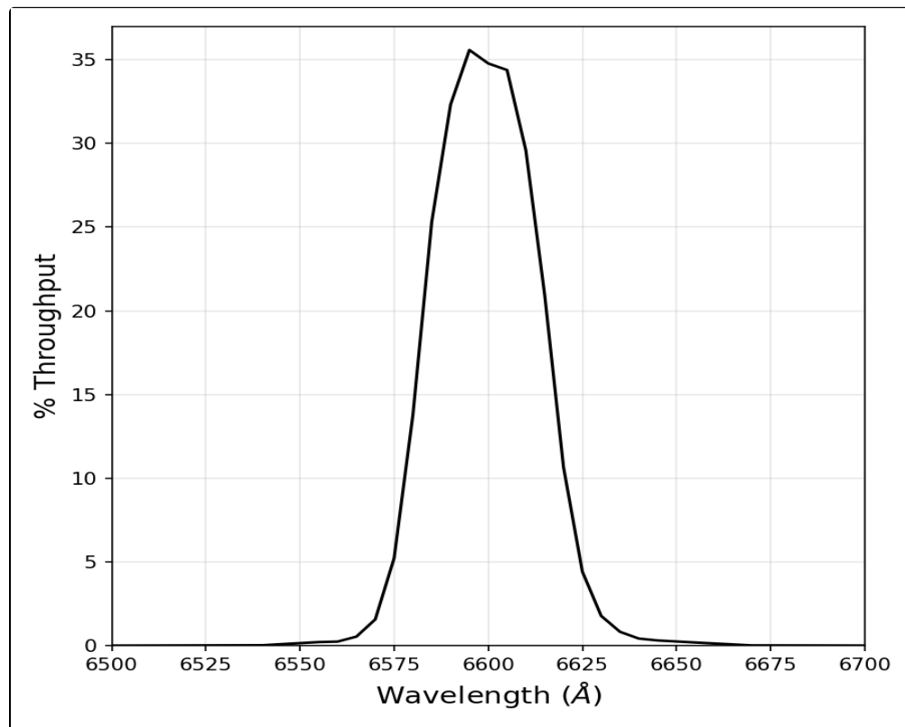
Figure 10.25: Integrated system throughput for WFC/F660N.
