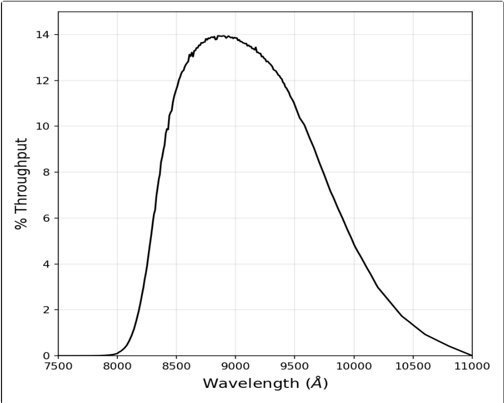
Figure 10.88: Integrated system throughput for HRC/F850LP.
