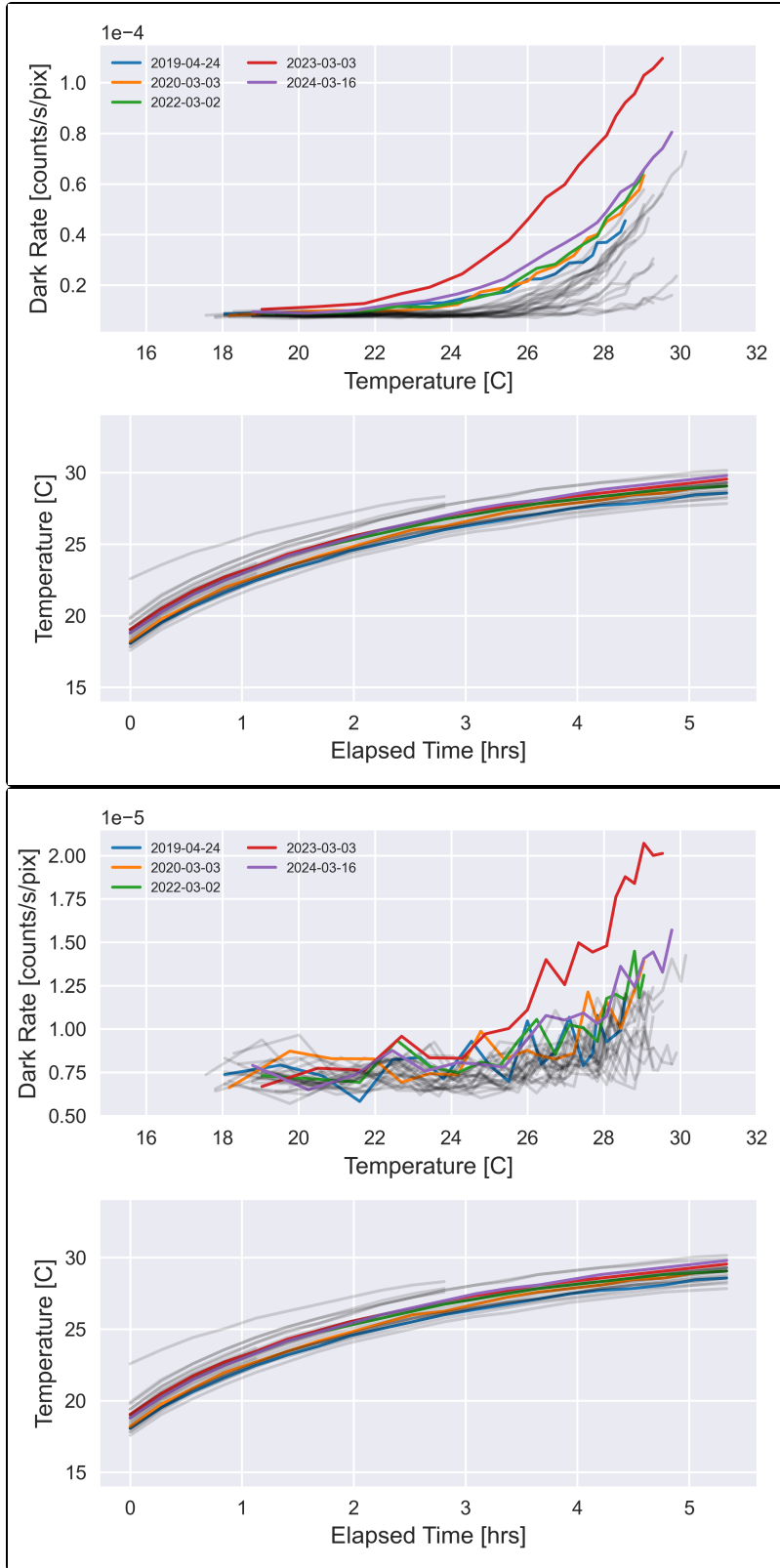
Figure 4.16: SBC Dark Rate and Operating Temperature.
