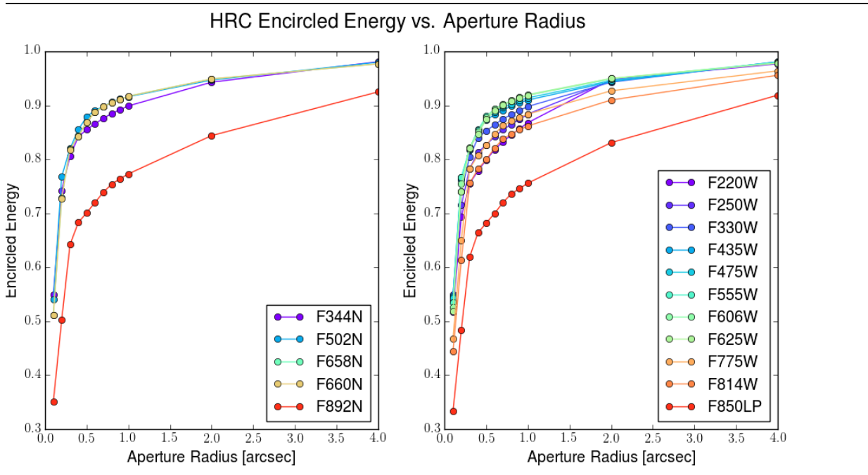
Figure 5.13: Encircled energy for the CCD channels.
