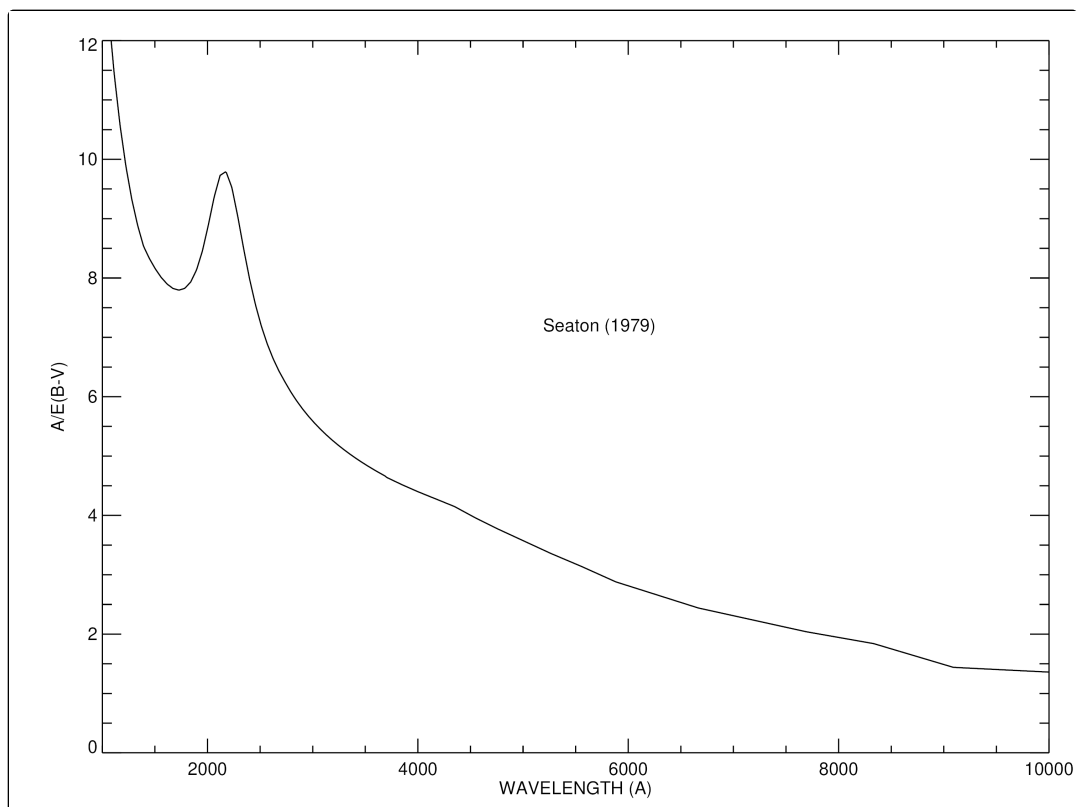
The mean UV interstellar extinction curve of the Milky Way as a function of wavelength. The curve features a prominent bump at 2200 \text{\AA} , which can disappear at lower metallicities.
