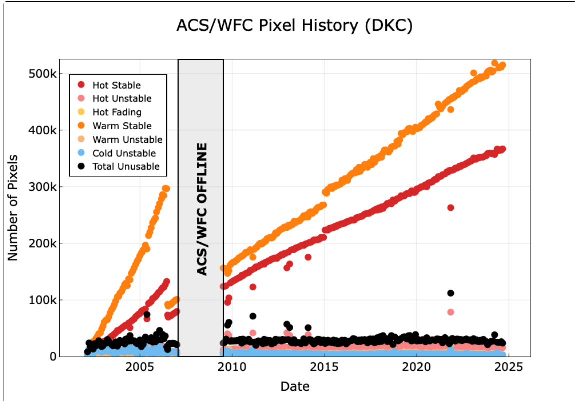
Figure 4.7: Pixel Stability and Hot Pixel Growth in WFC.
