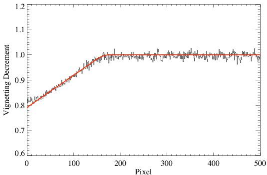
Figure 5.11: Vignetting Profile for NUV M Gratings.
