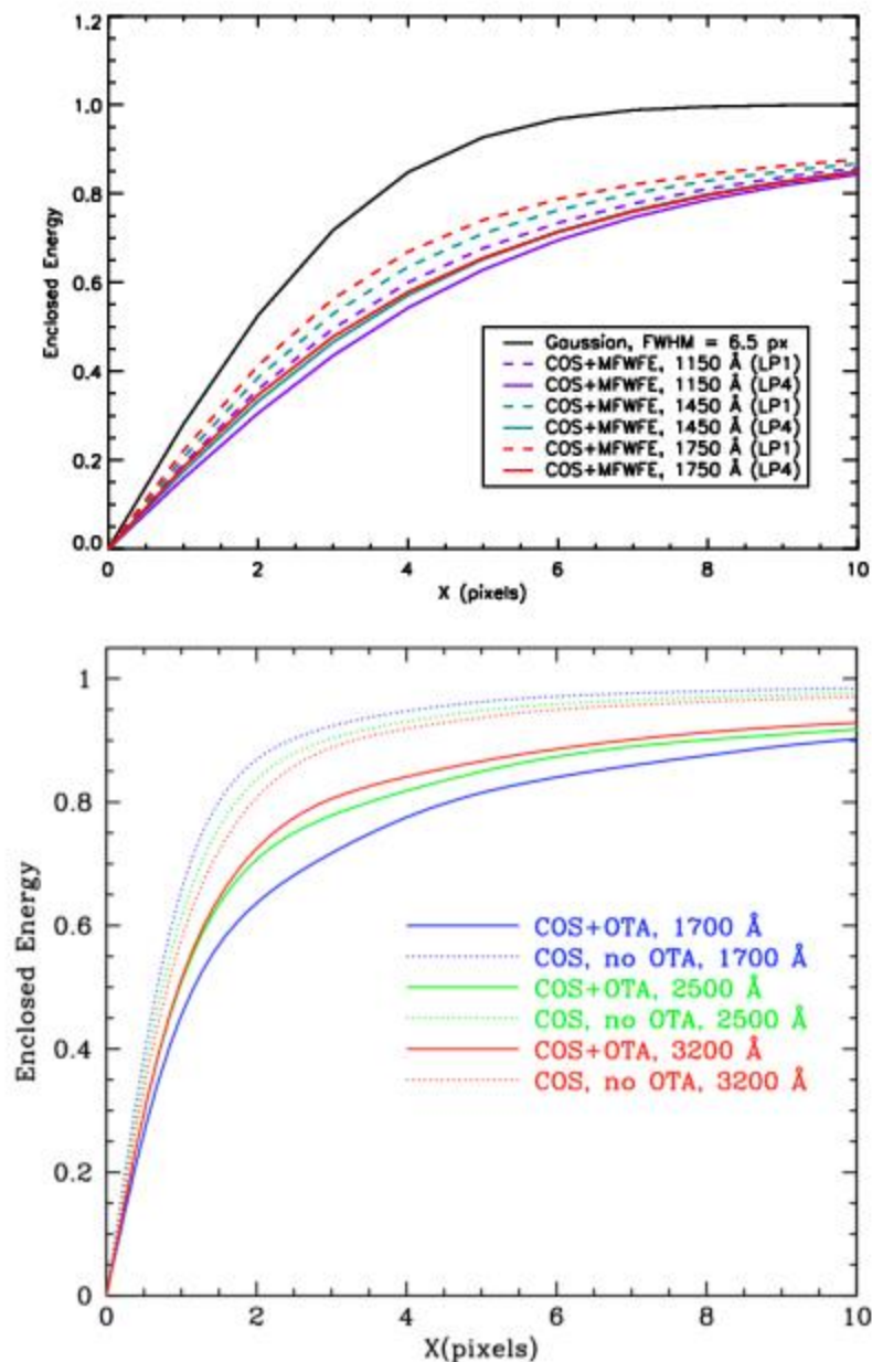
The enclosed energy fraction of the COS LSF for an unresolved spectral feature as measured from the center of the profile (collapsed along the cross-dispersion direction). The top panel shows a Gaussian with FWHM = 6.5 px and FUV model profiles. The 1150 Å data (purple) use the G130M grating, while the 1450 Å (teal) and 1750 Å (red) data use the G160M grating. The dashed lines indicate results for the original lifetime position, while the solid lines indicate data for the fourth lifetime position. In the bottom panel, NUV model profiles with and without the effects of the OTA MFWFEs are shown (Ghavamian et al. 2009). The 1700 Å data (blue) use the G185M grating, the 2500 Å data (green) use the G225M grating, and the 3200 Å data (red) use the G285M grating. Table 3.2: Distance from Line Center (in Pixels) versus Enclosed Energy Fraction and Wavelength for the G130M Grating. 1
